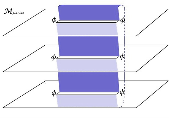
Figure 1: An artist's impression of the Riemann surface \mathcal{M}_{n,x_1,x_2} for n = 3 with field insertions \phi at the branch points x_1, x_2 .
