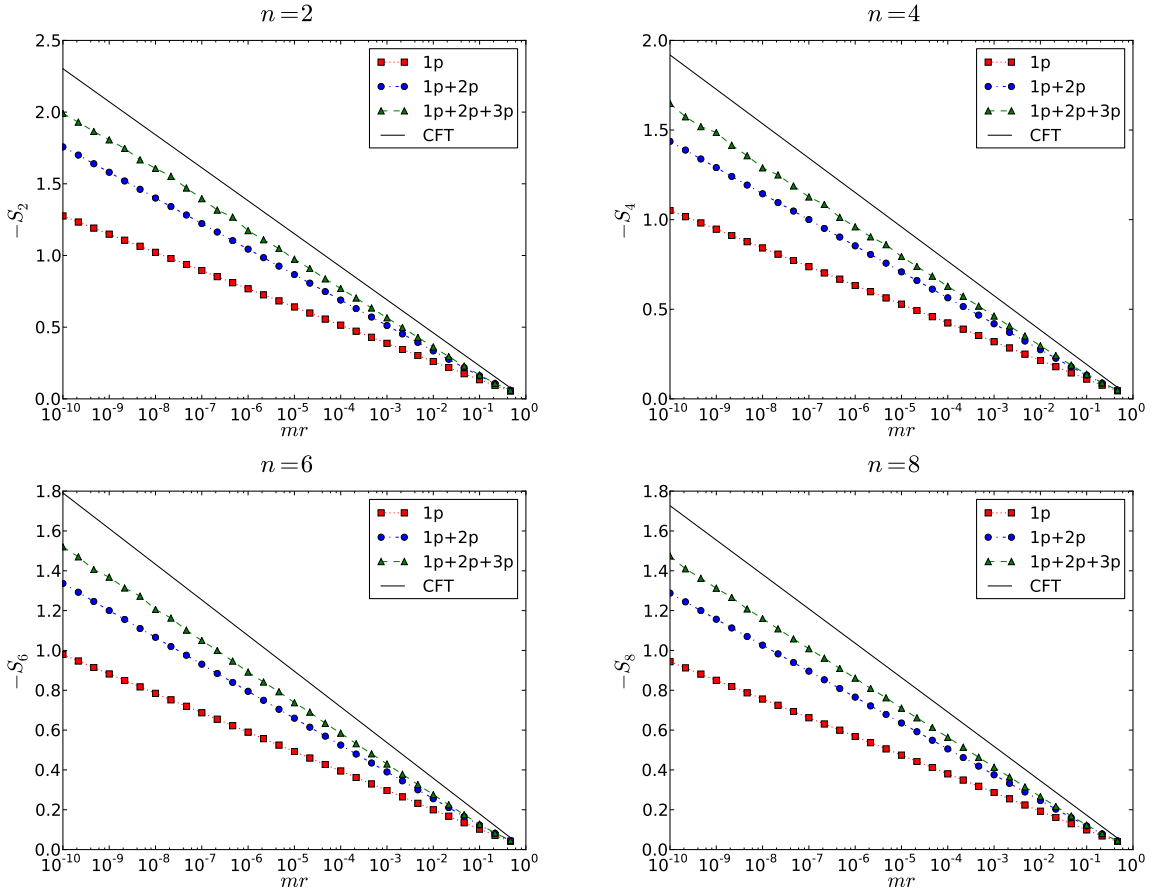
Figure 5: The Rényi entropy (3) with (14), subtracting the non-universal, positive, infinite additive contribution \frac{1}{1-n} \log \mathcal{Z}_n - \frac{c_{\text{eff}}}{6} \left(1 + \frac{1}{n}\right) \log(m\varepsilon) , and evaluated in logarithmic scale using form factors. The form factor contributions up to one-, two- and three-particles 1p are considered both for the correlators \langle : \mathcal{T}\phi : (r) : \tilde{\mathcal{T}}\phi : (0) \rangle and \langle \phi(r)\phi(0) \rangle . The solid line represents the CFT prediction \frac{c_{\text{eff}}(n+1)}{6n} \log(mr) (note that for mr < 1 , this is negative). All graphs show a clear logarithmic divergence at mr = 0 (as expected). Additional form factor contributions (also as expected) improve agreement with CFT.
