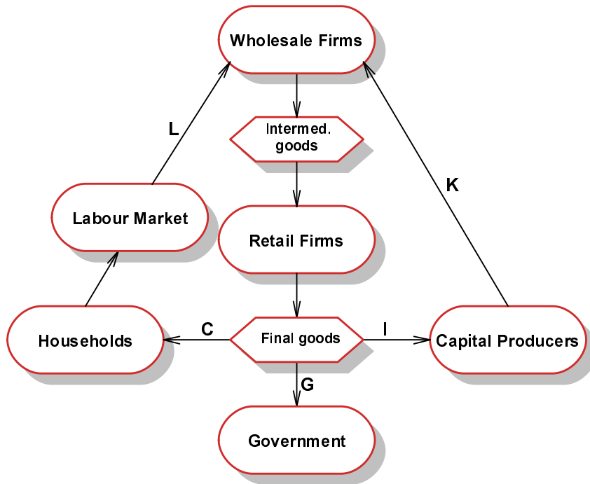
Figure 2: Model Structure
