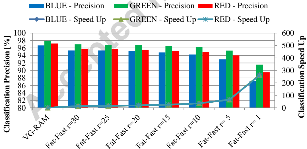
Figure 10: Traffic Sign Recognition System performance. Bars (blue, green, and red channels): Classification precision for implementations with standard VG-RAM, and Fat-Fast VG-RAM with different values of r for p/h = 8 bits. Curve: Speedup of the Fat-Fast implementation for different values of r .
