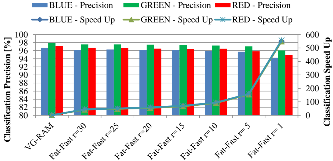
Figure 9: Traffic Sign Recognition System performance. Bars (blue, green, and red channels): Classification precision for implementations with standard VG-RAM, and Fat-Fast VG-RAM with different values of r for p/h = 16 bits. Curve: Speedup of the Fat-Fast implementation for different values of r .
