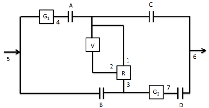
Figure 5 Dual-mode PSCVT
