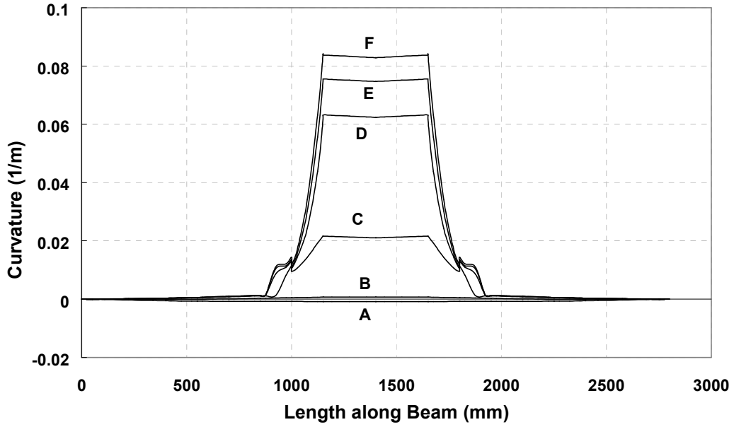
Figure 21 Curvature Distribution for Beam 16/65-1150
