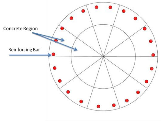
Fig. 9: Sample modelling of pier cross-section for the section-fibre analysis
