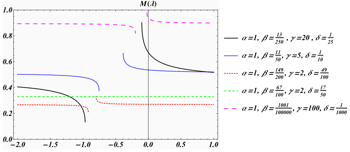
Figure 1: Modified mass M as a function of \lambda for m = 1 with \lambda \in \mathbb{R} \setminus (-0.9665, -0.0998) , \lambda \in \mathbb{R} \setminus (-0.7534, -0.3846) , \lambda \in \mathbb{R} \setminus (-0.9182, -0.8) , \lambda \in \mathbb{R} \setminus (-0.80709, -0.8) and \lambda \in \mathbb{R} \setminus (-0.1978, -0.0200) .
