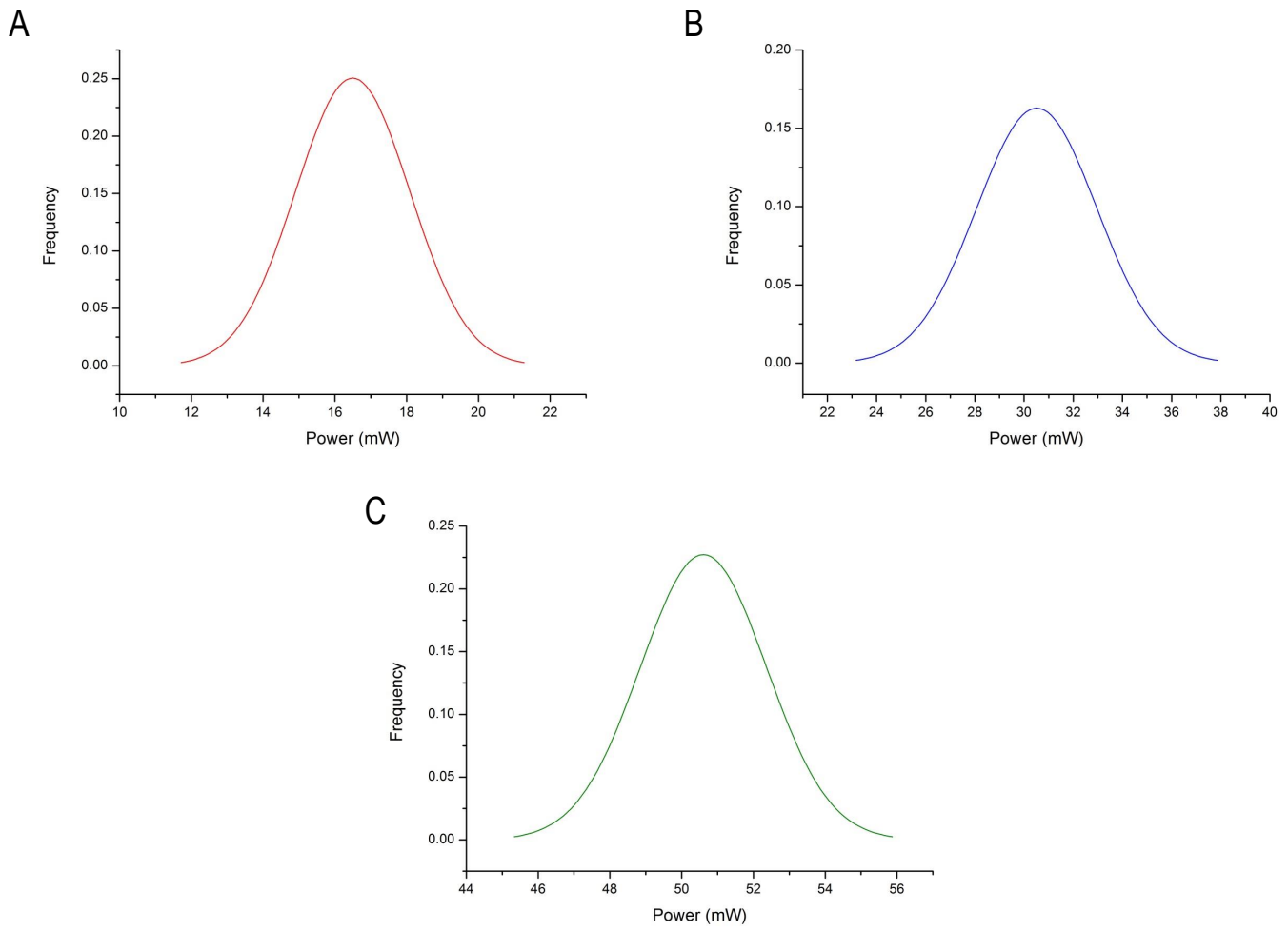
Figure 3.21: Normal Distribution for Power Measurements of Model 1 Mechanism Only; A: 5 Hz, B: 8 Hz and C: 12 Hz
