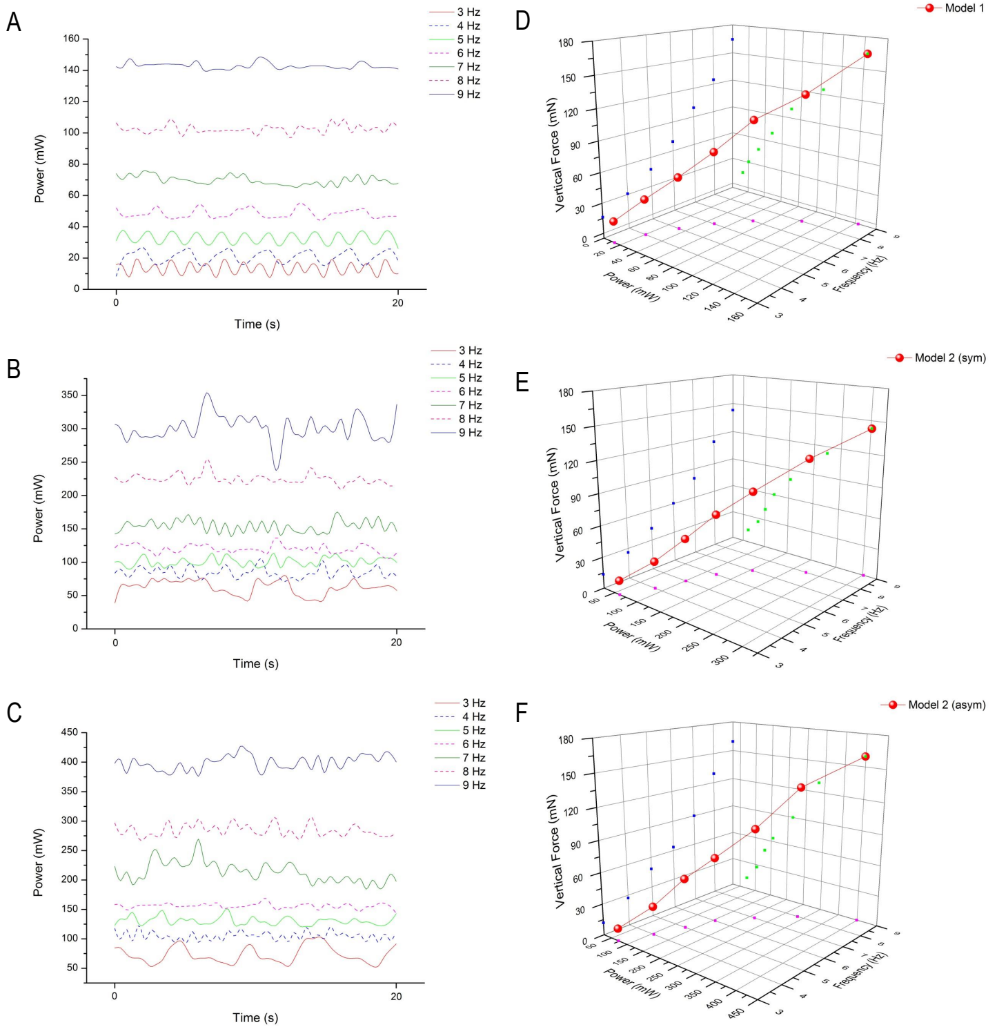
Figure 3.22: Power and Force Measurements of 52 mm Carbon Fibre Bar Flapping; A: Model 1, B: Model 2 (sym), C: Model 2 (asym), D: Model 1, E: Model 2 (sym), F: Model 2 (asym), Coloured Dots in Graphs D,E,F Represent Axes Projections Such as Blue: Frequency Vs Vertical Force, Magenta: Frequency Vs Power, Green: Power Vs Vertical Force
