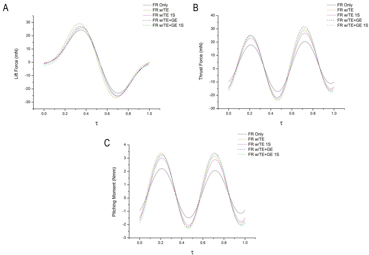
Figure 6.17: Flapping & Rotation Wing Measurements for 60 mm Wings (WT 4 ); A: Comparison of Lift Force, B: Comparison of Thrust Force, C: Comparison of Pitching Moment. UI: M1-FR-WT 4 -S-V & M1-FRwB-WT 4 -S-V
