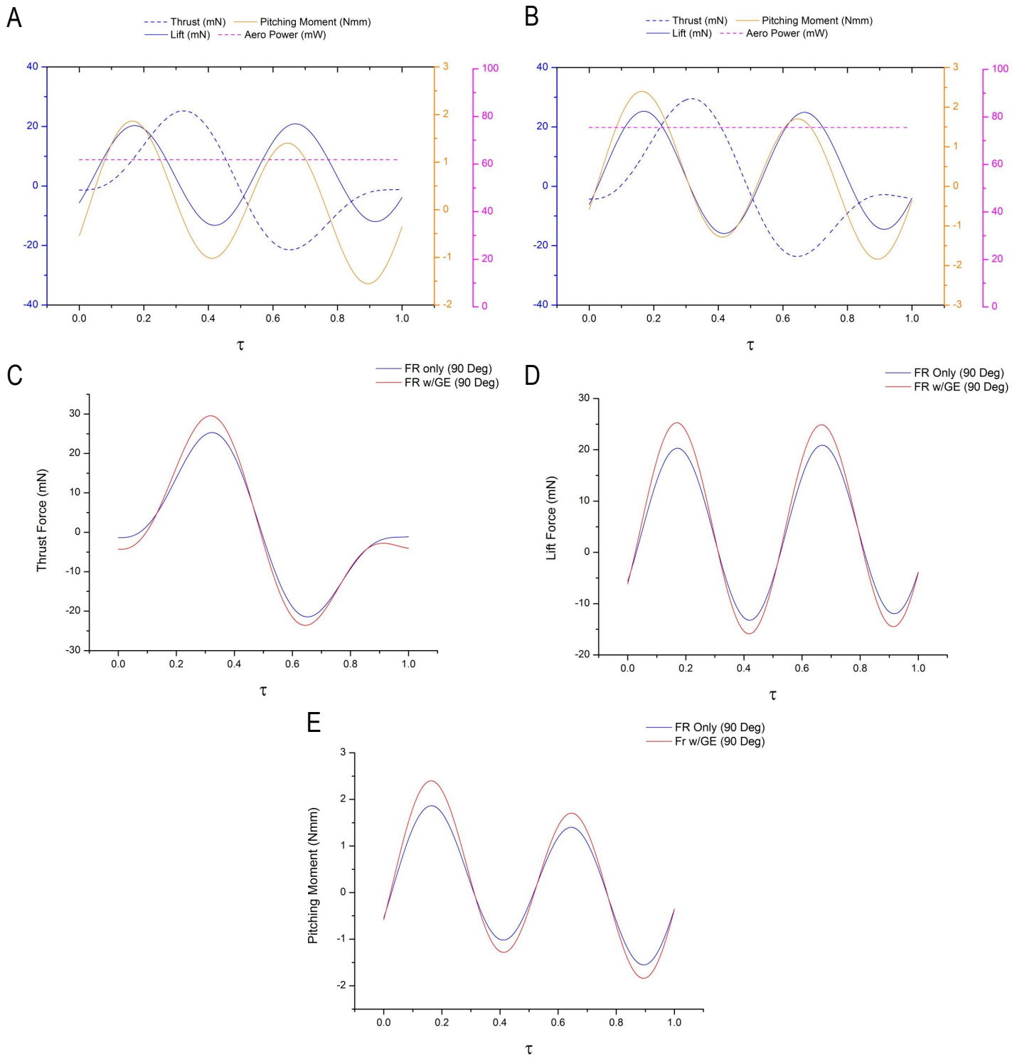
Figure 6.19: Flapping & Rotation Wing Measurements for 60 mm Wings (WT 4 ) with Model in Hovering Position; A: FR Only (90 Deg), B: FR w/GE Boundary (90 Deg), C: Comparison of Thrust Force, D: Comparison of Lift Force, E: Comparison of Pitching Moment. UI: M1-FR-WT 4 -S-H & M1-FRwB-WT 4 -S-H
