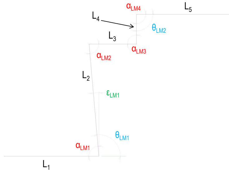
Figure 3.12: Linkage Mechanism in Neutral Position with Angles
