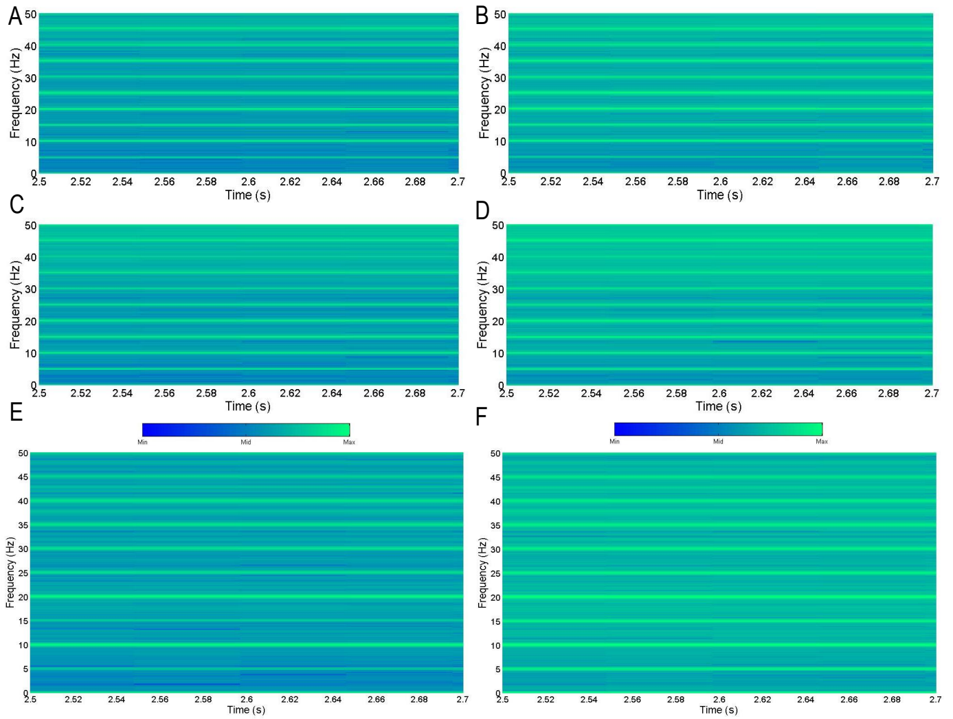
Figure B.1: Spectrogram Plots for 60 mm Wings ( WT_4 ) in FR & FRAP Configurations; A: FR for Fx Axis, B: FR for Ty Axis, C: FRAP for Fx Axis, D: FRAP for Ty Axis, E: FR in Hovering Mode for Fx Axis, F: FR in Hovering Mode for Ty Axis. Colour Bar Represents Size of Amplitude. UI: M1-FR- WT_4 -S-V, M1-FR- WT_4 -S-H & M1-FRAP- WT_4 -S-V
