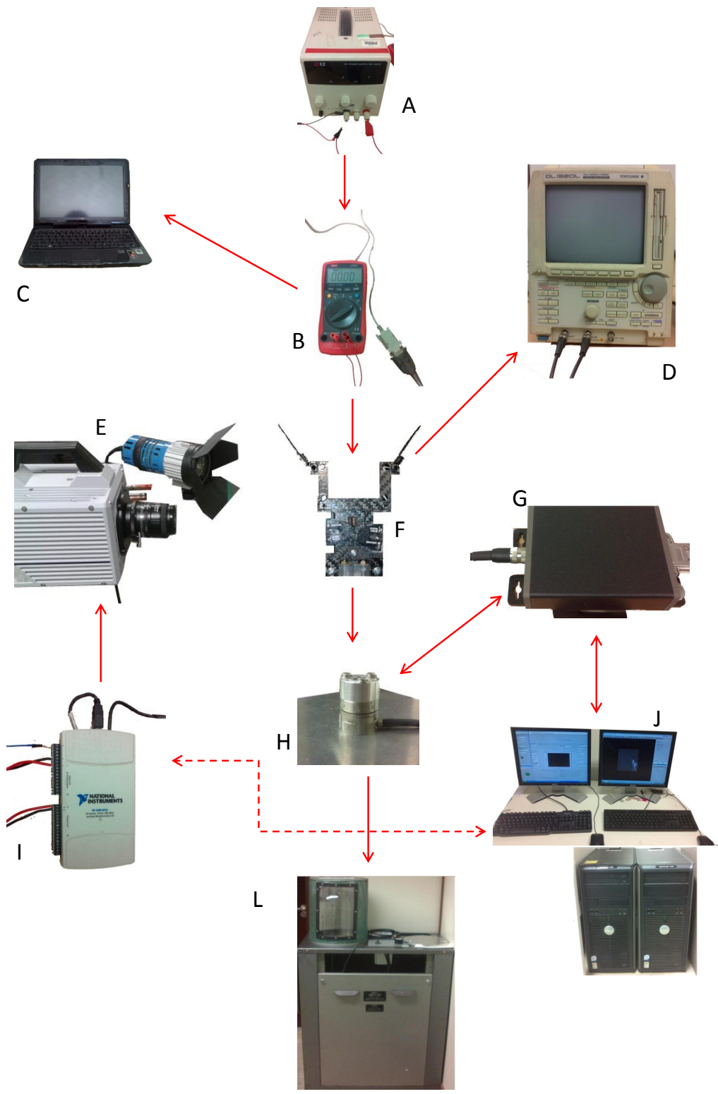
Figure 4.2: Schematic of Vacuum Chamber Tests
