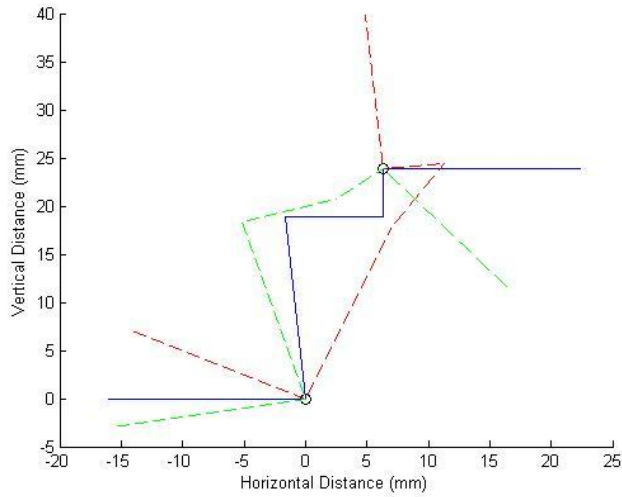
Figure 3.14: Linkage Mechanism in Three Different Positions; Blue: Neutral Position, Red: Start Downstroke Position, Green: Start Upstroke Position
