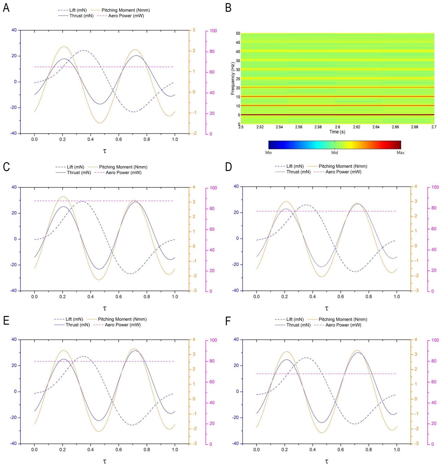
Figure 6.16: Flapping & Rotation Wing Measurements for 60 mm Wings (WT4); A: Case FR1, B: Spectrogram for Vertical Axis in Air, C: Case FR2, D: Case FR3, E: Case FR4, F: Case FR5. Colour Bar Represents Size of Amplitude. UI: M1-FR-WT4-S-V & M1-FRwB-WT4-S-V
