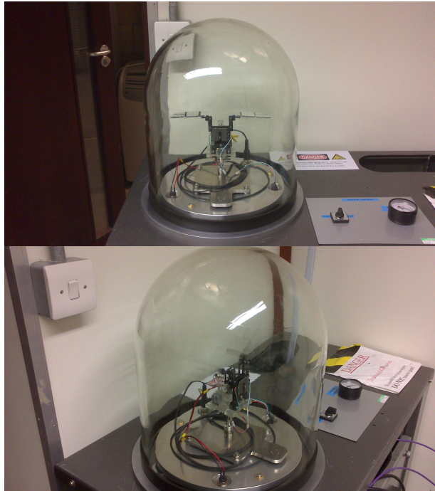
Figure 4.57: Photograph of Vac Chamber with Model at 0 Degree Body Inclination with 60 mm Wings (WT4)
