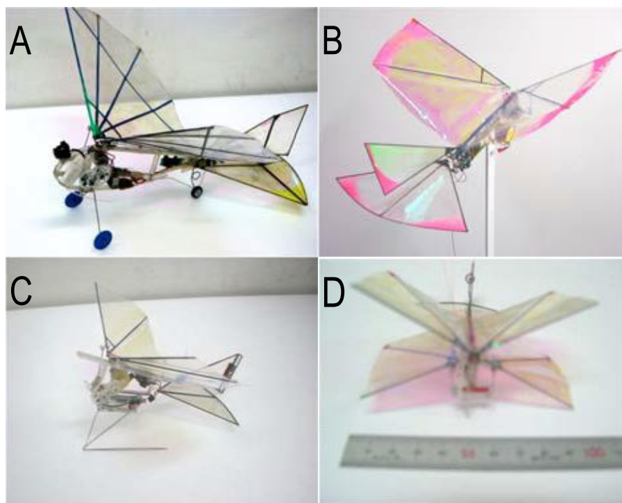
Figure 1.22: Konkuk Ornithopters & MAVs; A: 360 mm Wing Span; B: 280 mm Wing Span; C: 150 mm Wing Span; D: 100 mm Wing Span (Park et al. 2008)
