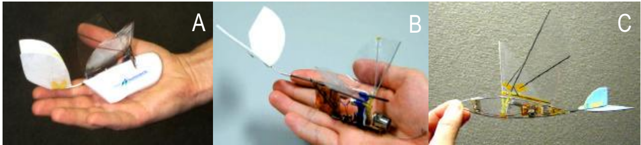
Figure 1.20: Microbat ; A: Super Capacitor Powered ; B: Battery Powered ; C: Battery Powered with R/C Navigation (Pornsir-Sirirak et al. 2001)
