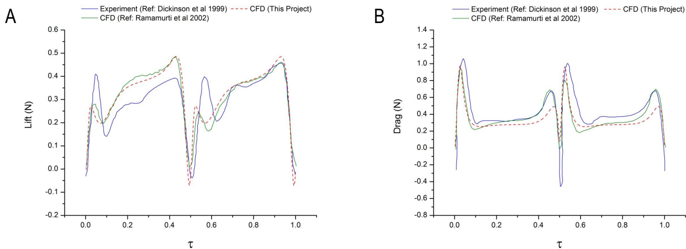
Figure 5.7: Drosophila Wing Measurement Comparison; A: Lift Force Comparison, B: Drag Force Comparison
