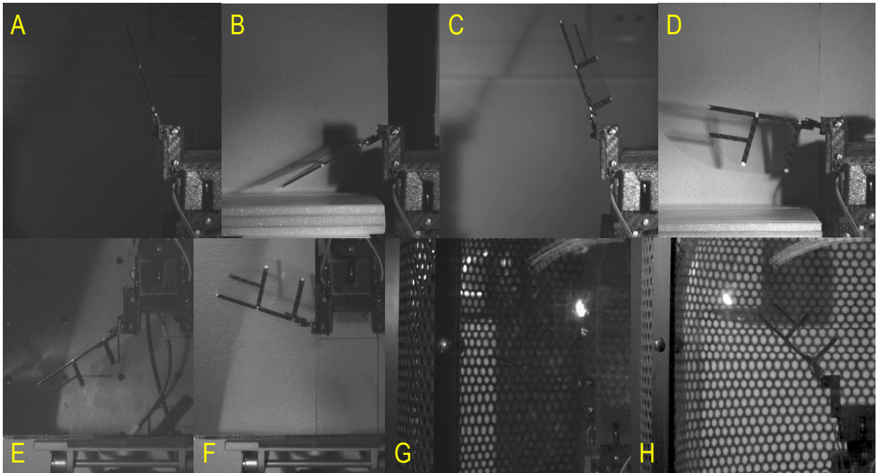
Figure B.3: Example of Experimental Images to Capture Wing Motion with Various Arrangements; A: Flapping Only, B: Flapping with TE wall and GE Boundaries, C: FR Only, D: FR with TE wall and GE Boundaries, E: FR Only in Hovering Mode, F: FR in Hovering Mode with GE Boundary, G: Flapping Only in Vacuum Chamber, H: FR Only in Vacuum Chamber
