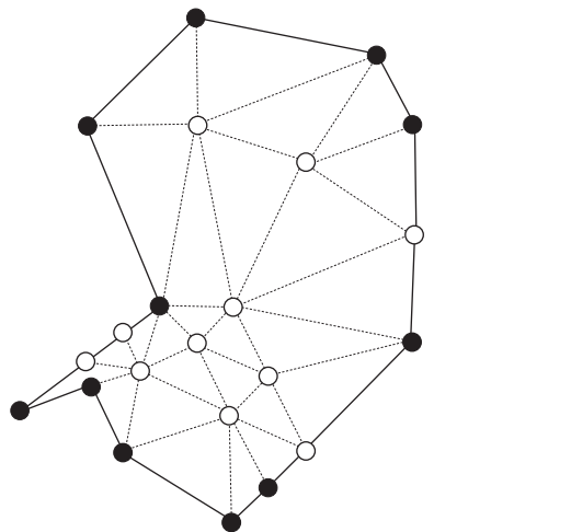
Fig. 16. Example of a 2D triangulation problem, the input data are represented by the solid vertices and edges and the obtained triangulation is given by the hollow vertices and dashed edges
