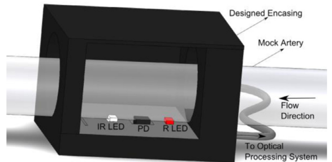
Fig. 3. 3D illustration of the custom-made PPG optical sensor enclosing a tube section, showing Infrared (IR) and Red (R) LEDs, a photodiode (PD), mock artery and the designed encasing.
