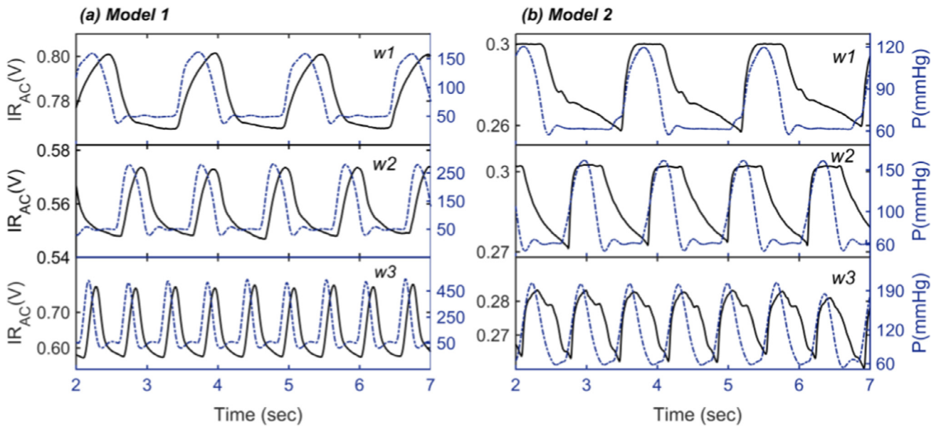
Fig. 7. 5 s sample for Infrared signals (IRAC) acquired from Model 1 and Model 2 . Pressure signals (P) are also plotted against the right y-axis. This set of data is acquired at 70 ml of stroke volume at all operated pulse frequencies; (a) Signals acquired from Model 1 .at a stroke volume of 70 ml and all operating frequencies; (b) Shows signals acquired from Model 2 at a stroke volume of 70 ml and all operating frequencies.
