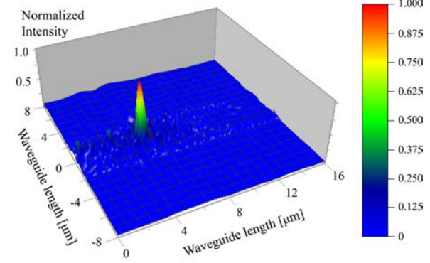
Figure 2: The Optiwave results, where the parameters are R_l = R_r = 1.2 \mu\text{m} , R_d = 2.0 \mu\text{m} , R_{Si} = R_{Gr} = 1.0 \mu\text{m} , R_{Au} = 10 \text{ nm} , h_{Au} = 200 \text{ nm} , the thickness of Si and Graphene is 1 \mu\text{m} and 10 \text{ nm} , respectively, the input light power is 200 mW. The refractive index of the silicon is 1.46. The linear and nonlinear refractive indices of the GaAsInP/P are 3.14 and 1.30 \times 10^{-13} \text{ m}^2 \text{ W}^{-1} , respectively. The attenuation coefficient of the waveguide is 0.1 \text{ dB} (\text{mm})^{-1} .
