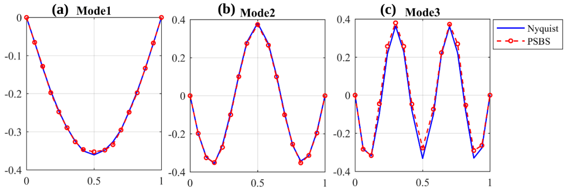
Figure 5.30: Nyquist FDD versus PSBS-based FDD at CR=31% for mode shape estimation at DS0 for SNR=10dB (the horizontal axis gives the relative distance from the left support of the beam normalised with its length)
