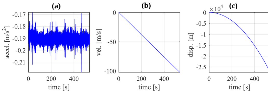
Figure 6.10: Typical acceleration-velocity-displacement time series recorded at sensor #13 pertaining to the raw data
