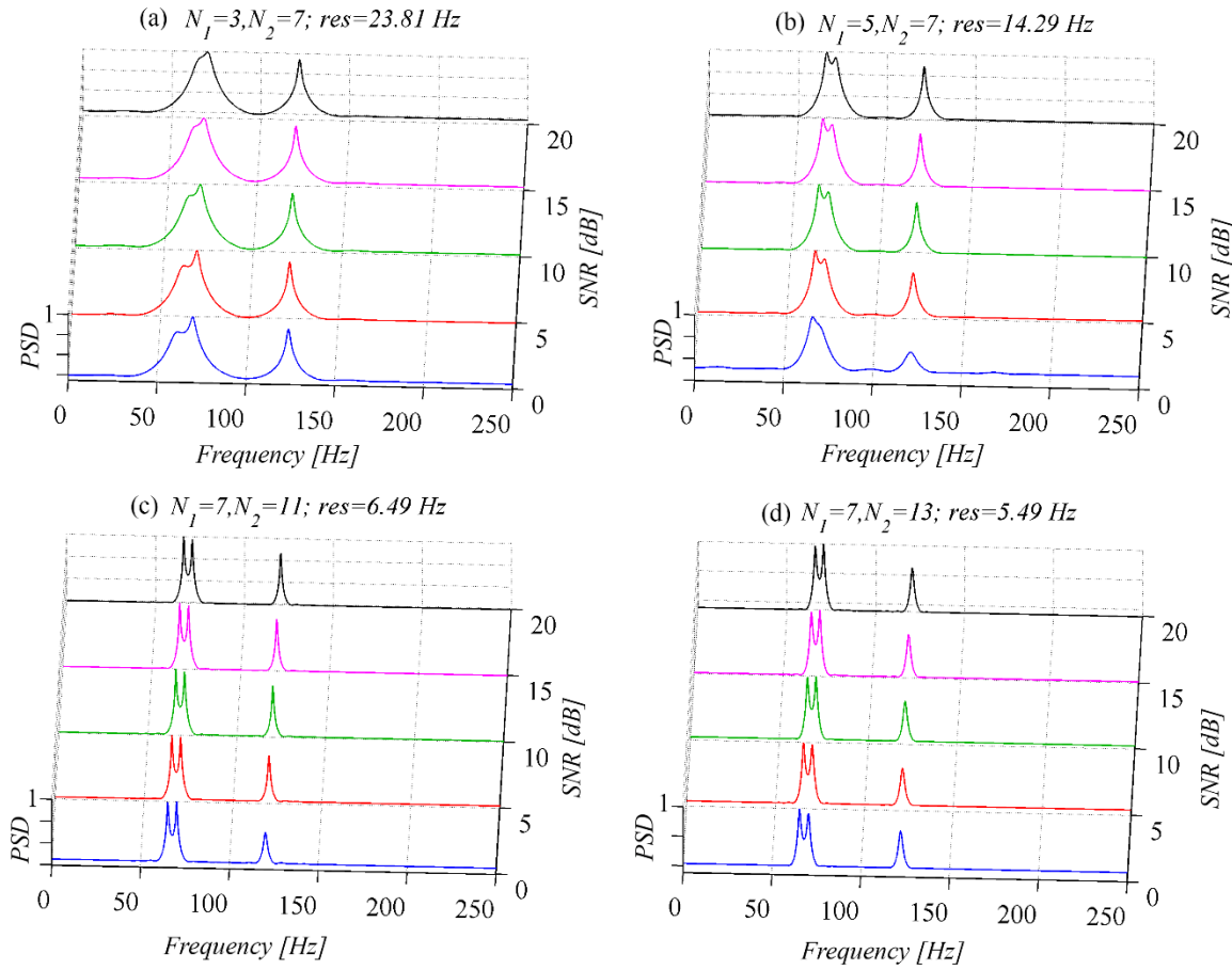
Figure 7.3: Parametric analysis with respect to SNR for the MUSIC and co-prime method for df/f=6\% ( f_1=66\text{Hz} , f_2=70\text{Hz} ); (a) N_1=3 , N_2=7 , resolution 23.81Hz (b) N_1=5 , N_2=7 , resolution 14.29Hz (c) N_1=7 , N_2=11 , resolution 6.49Hz (d) N_1=7 , N_2=13 , resolution 5.49Hz
