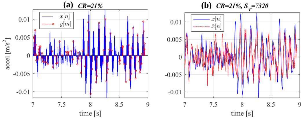
Figure 6.16: (a) Compressive sensing at CR=21% and the acquisition of M=82 samples within a time-window of 2sec duration with N=400 Nyquist samples and (b) CoSaMP-based signal reconstruction of acceleration response signal at sensor #13 for S_T=7320 .
