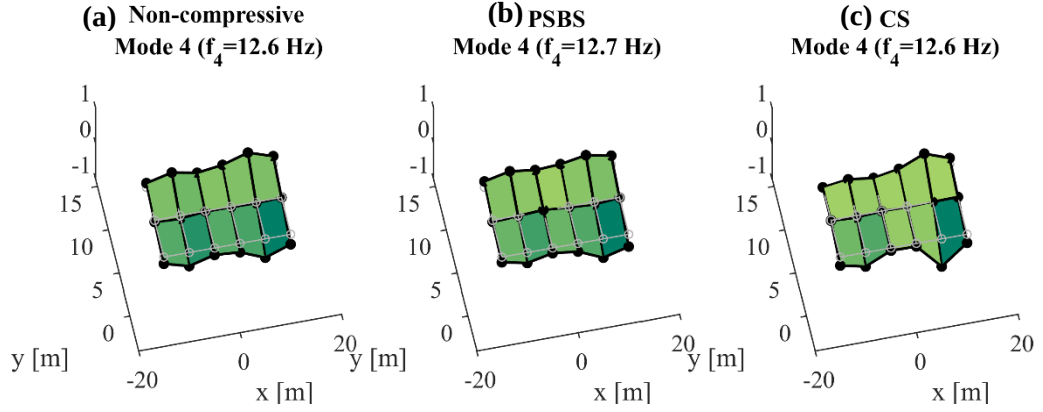
Figure 6.22: Estimation of the 4 th mode shape (rotational) of the Bärenbohlstrasse bridge; (a) conventional/non-compressive FDD; (b) PSBS-based FDD at CR=11%; and (c) the CS-based approach for CR=11% and target reconstruction sparsity S_T=3840 .
