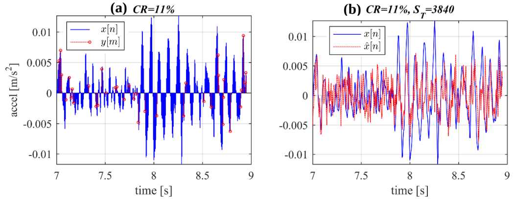
Figure 6.17: (a) Compressive sensing at CR=11% and the acquisition of M=44 samples within a time-window of 2sec duration with N=400 Nyquist samples and (b) CoSaMP-based signal reconstruction of acceleration response signal at sensor #13 for S_T=3840 .
