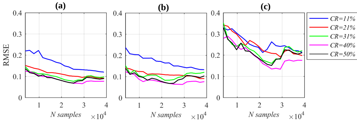
Figure 5.7: RMSE versus observation's window length, N , for the 1 st case study with \omega_1=20\text{rad/s} and \omega_2=60\text{rad/s} : (a) RMSE in the wide-band range of [0-100 \text{ rad/s}] ; (b) RMSE in the narrow-band range of [10-30] \text{ rad/s} (around \omega_1 ); (c) RMSE in the narrow-band range of [50-60] \text{ rad/s} (around \omega_2 )
