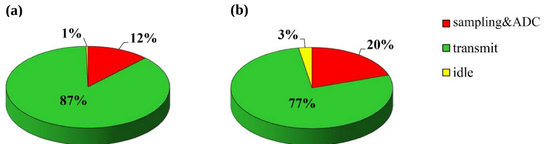
Figure 6.28: Energy distribution in the various sensor activities for (a) the conventional sampling with CR=77.6\% off-line lossless compression and (b) the multi-coset sampling scheme with CR=11\% for the bridge case study
