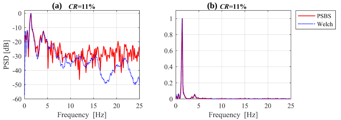
Figure 5.18: PSD estimates: Welch periodogram at Nyquist rate compared with PSBS approach for CR=11\% ( M=14, \bar{N}=128 ) in (a) logarithmic scale, and (b) linear scale
