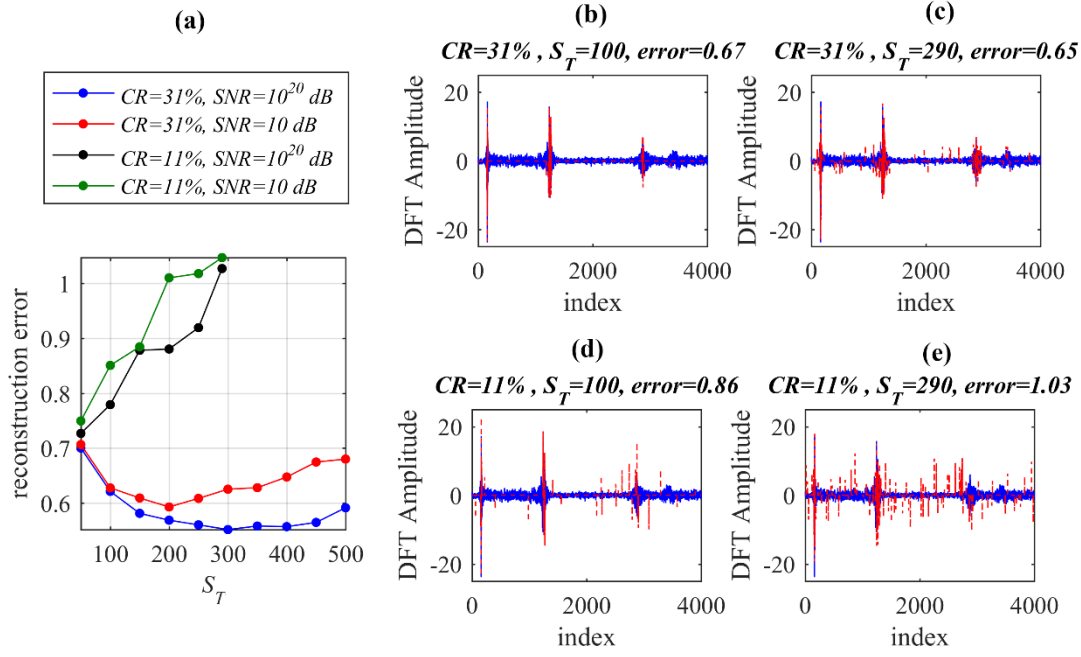
Figure 6.3: (a) Signal reconstruction error of CoSaMP algorithm versus the target sparsity level S_T ; (b-e) original and reconstructed DFT coefficients at CR=\{31\%,11\%\} , S_T=\{100, 290\} for SNR=10 dB
