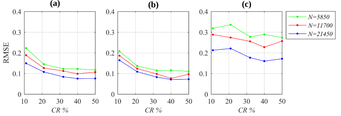
Figure 5.8: RMSE versus CR for the 1 st case study with \omega_1=20\text{rad/s} and \omega_2=60\text{ rad/s} : (a) RMSE in the wide-band range of [0-100\text{ rad/s}] ; (b) RMSE in the narrow-band range of [10-30]\text{ rad/s} (around \omega_1 ); (c) RMSE in the narrow-band range of [50-60]\text{ rad/s} (around \omega_2 )
