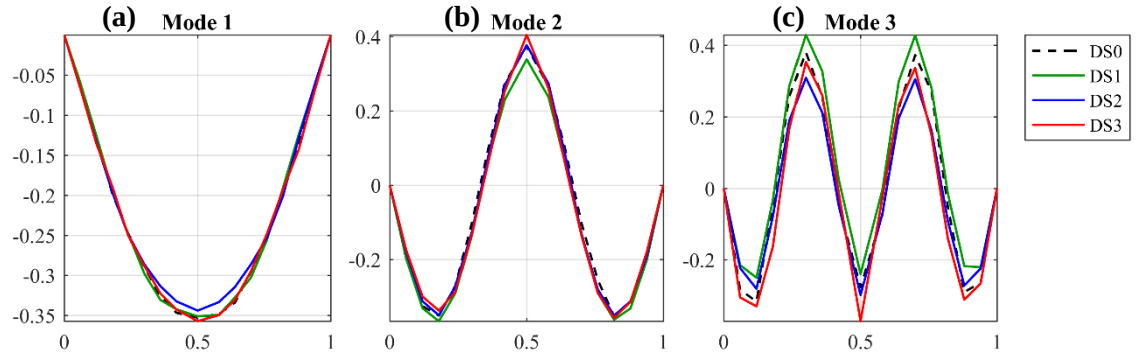
Figure 5.29: PSBS-based FDD at CR=31% for mode shape estimation at DS0-DS3 for SNR=10dB (the horizontal axis gives the relative distance from the left support of the beam normalised with its length)
