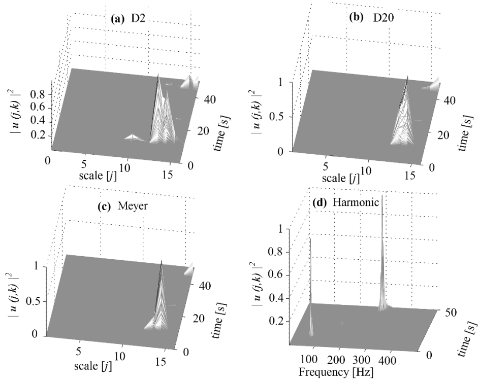
Figure 3.11: Normalised squared magnitude of wavelet coefficients pertaining to the truss acceleration response at node #4 (damaged state) under the sine-sweep excitation; discrete wavelet transform analysis with (a) D2 (Haar), (b) D20, (c) Meyer; and (d) Harmonic wavelet transform
