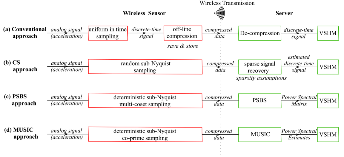
Figure 1.1: Comparison of four different data acquisition schemes in wireless sensors for VSHM: (a) conventional; (b) CS-based; (c) PSBS-based; and (d) co-prime based approach
