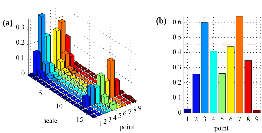
Figure 3.19: (a) Scale-dependent RWE(j) in eq. (3.18) and (b) RWE in eq. (3.10) using the Meyer wavelet filter bank for the space truss subject to the white noise excitation.
