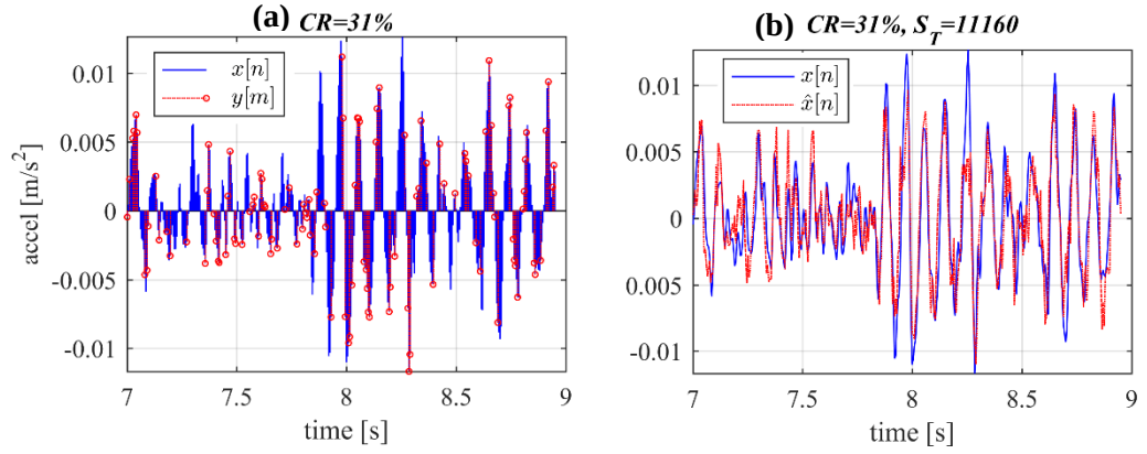
Figure 6.15: (a) Compressive sensing at CR=31% and the acquisition of M=125 samples within a time-window of 2sec duration with N=400 Nyquist samples and (b) CoSaMP-based signal reconstruction of acceleration response signal at sensor #13 for S_T=11160 .
