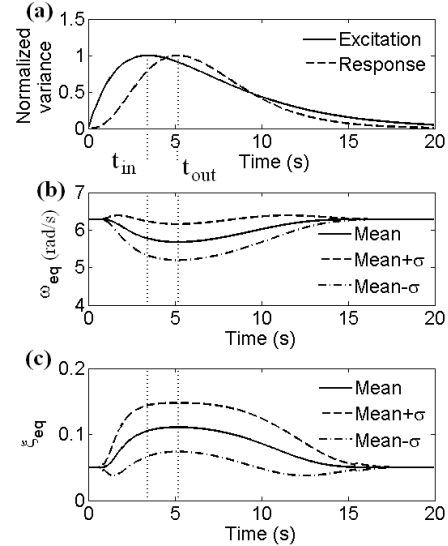
Figure 4: (a) Excitation (acceleration) and response (deflection) variances normalized to their peak values; (b) and (c) ELPs for bilinear oscillator with a= 0.5 , \omega_o= 2\pi rad/s, \xi_o= 5\% , and u_y= 6 cm.
