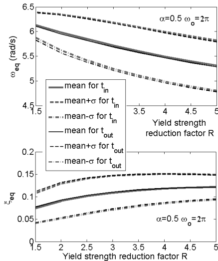
Figure 5: ELPs for bilinear oscillator with a=0.5 , \omega_o=2\pi rad/s, and various yielding displacement u_y
