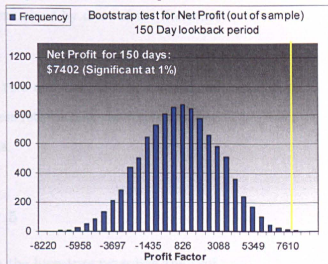
Figure 5.9: Out-of-sample Results for Net Profit.
