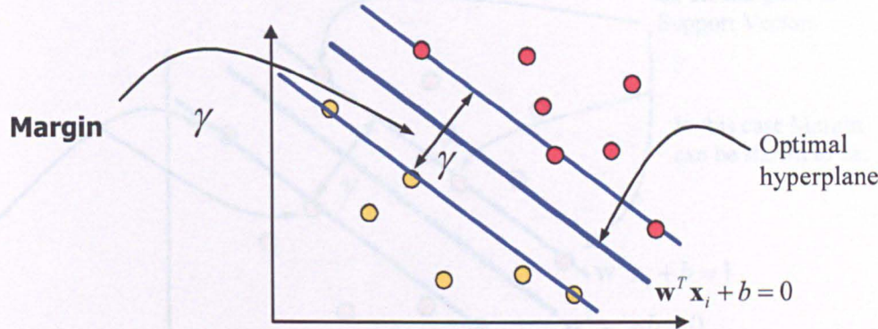
Figure 2.3: Hyperplane & Margin
