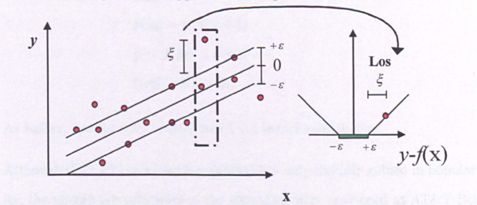
Figure 2.7: Support vector regression & the tube
