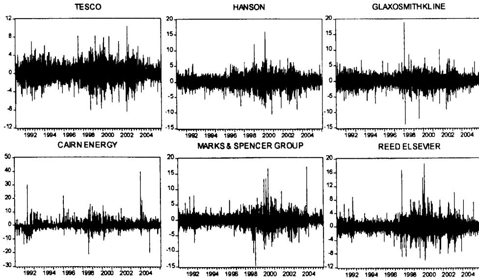
Figure 4.2: Log returns of six of 65 stocks.
