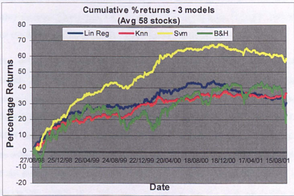
Figure 3.4: Cumulative percentage returns 3 Models
