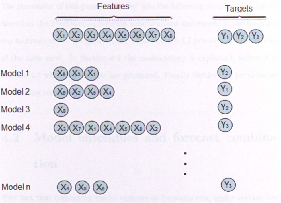
Figure 4.1: Random Subspace Method
