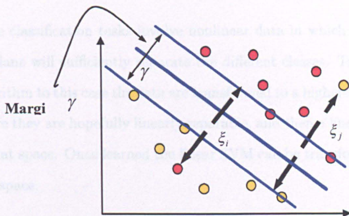
Figure 2.5: Introduction of slack variables.
