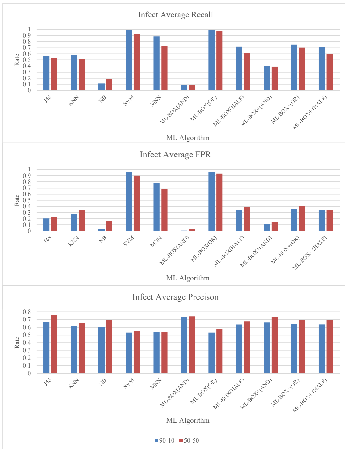
Figure 4-14 - Comparison of ML algorithms
