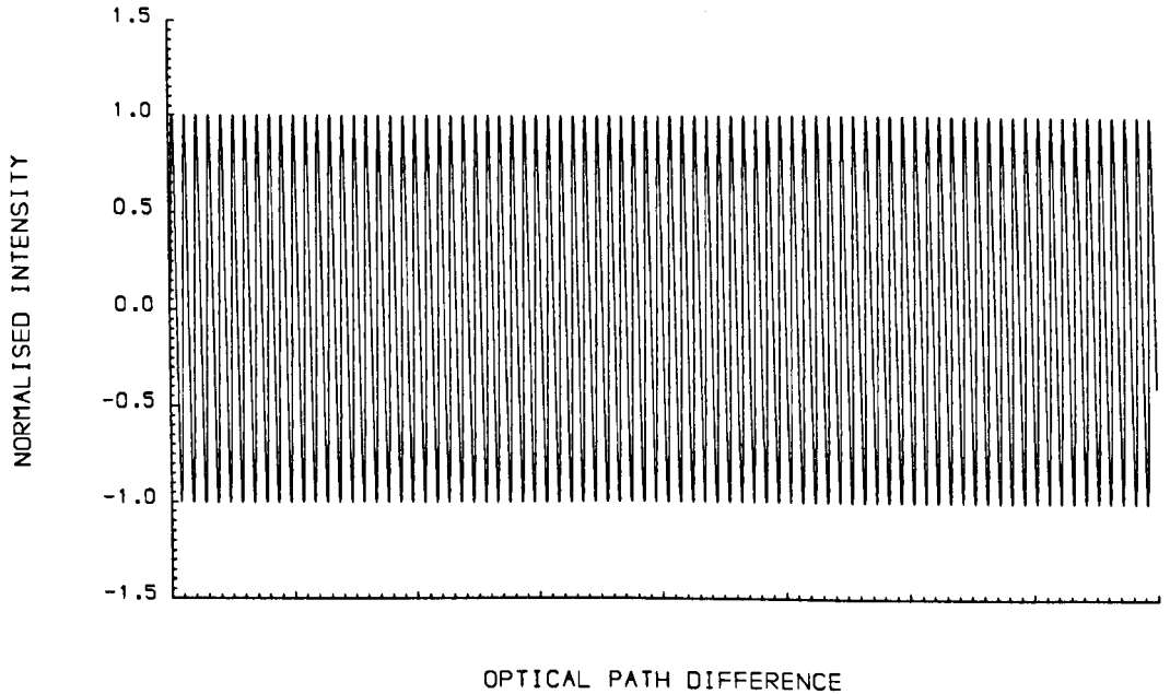
Fig. 1.1 Output intensity with a He-Ne laser source. L_c = 1000 \text{ m} , corresponding to 1.58 \times 10^9 fringes.
