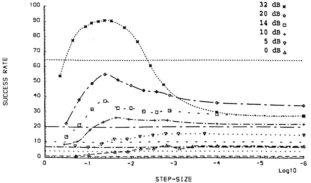
Fig. 5.1 Success rate with the thresholded technique against \mu and SNR, with p = 32 . The horizontal lines refer to the direct visibility method.
