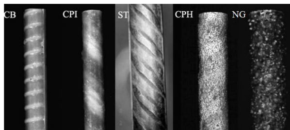
Figure 1. Tested re-bars.
