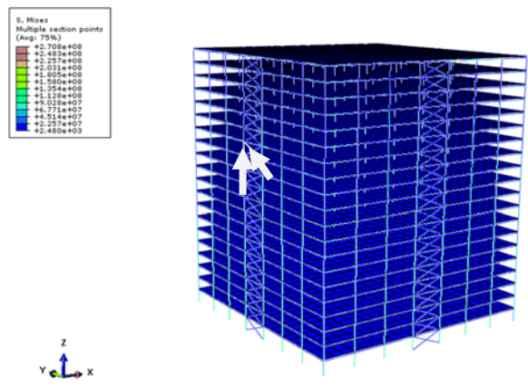
Fig .22 Von mises stress contour of case 5
