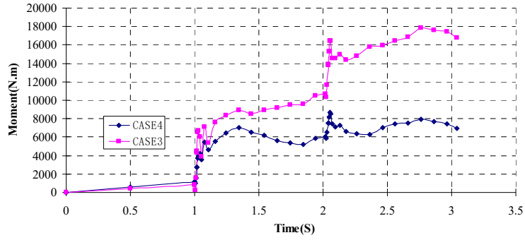
Fig.26 Major bending moment of beam B1A1 at ground level for case 3 and at level 14 for case 5
