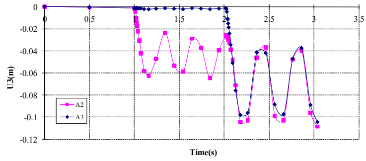
Fig.29 Displacement of the node at A2 and A3 of Case 1
