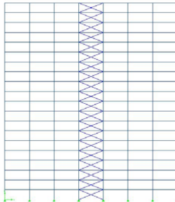
Fig 2 elevation of 20-story prototype building
