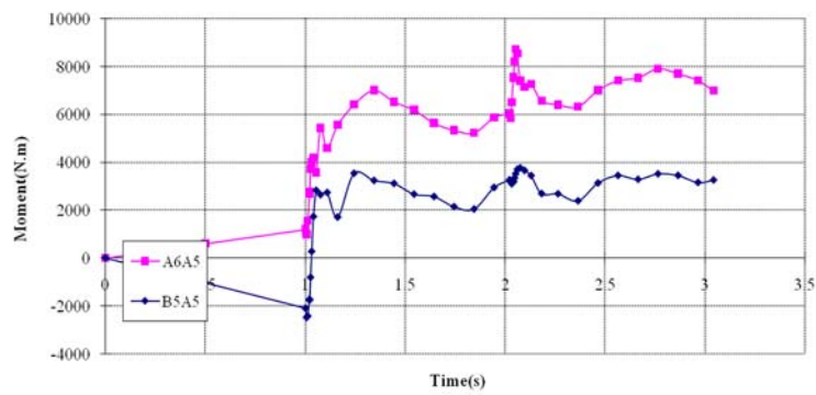
Fig.24 Major bending moment of Beam A6A5,B5A5 at level 14 of Case 5
