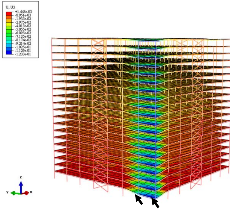
Fig.3 Vertical displacement of case 1 (deformation scale factor 10)
