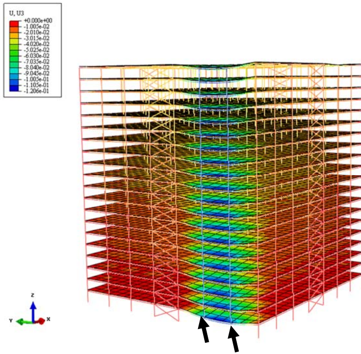
Fig .27 Vertical displacement contour of case 6
