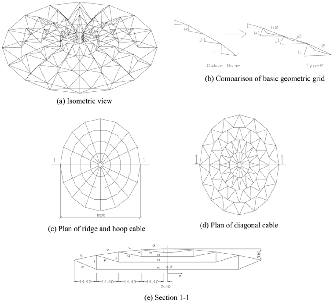
Fig. 12 Structural Type 2
