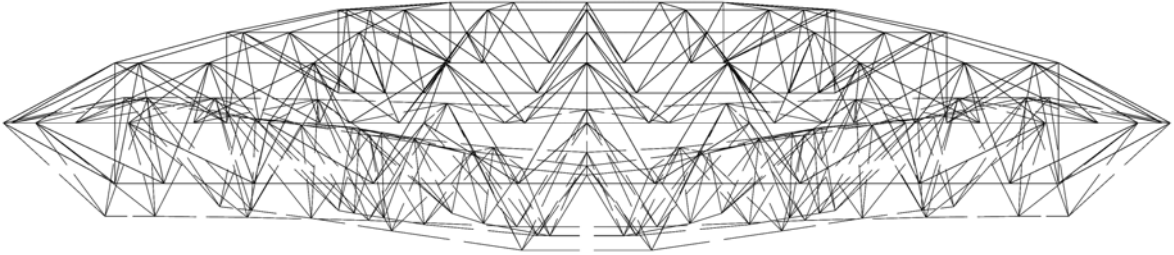
Fig. 16 Deformation of the proposed model (100 times amplified from the original size)
