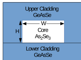
FIG. 1: Channel waveguide geometry.
