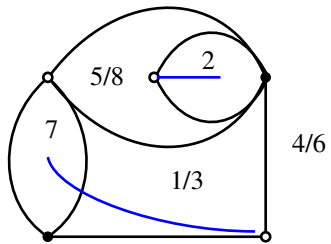
(I1) Map (3.7), defined over \mathbb{Q}(\sqrt{10}) .
