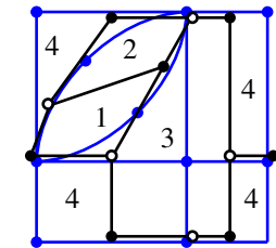
(L) Map (5.4) on (5.6), with \sqrt{-2} .
