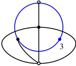
(N) Map (5.8) on a j = 0 curve.
