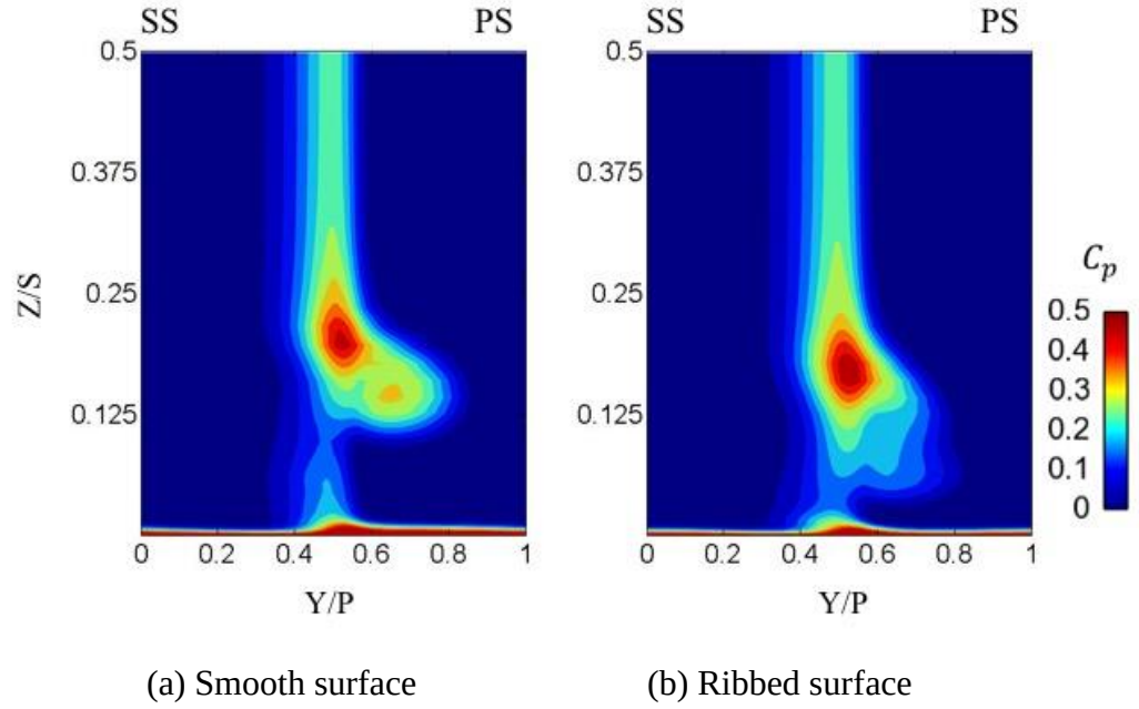
Figure 5.18: Aerodynamic loss coefficient C_p distributions obtained at 0.12 chord downstream of the cascade blade.
