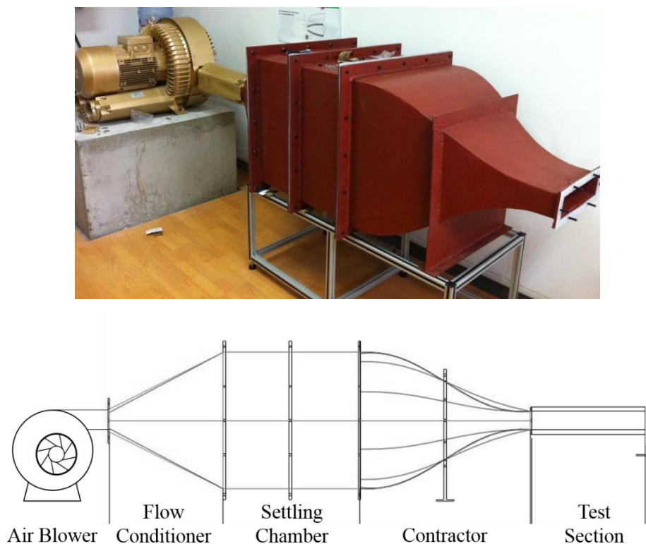
Figure 3.1: Low-speed wind tunnel
