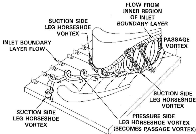
Figure 2.6: Secondary flow model of Sharma and Butler. (1986)
