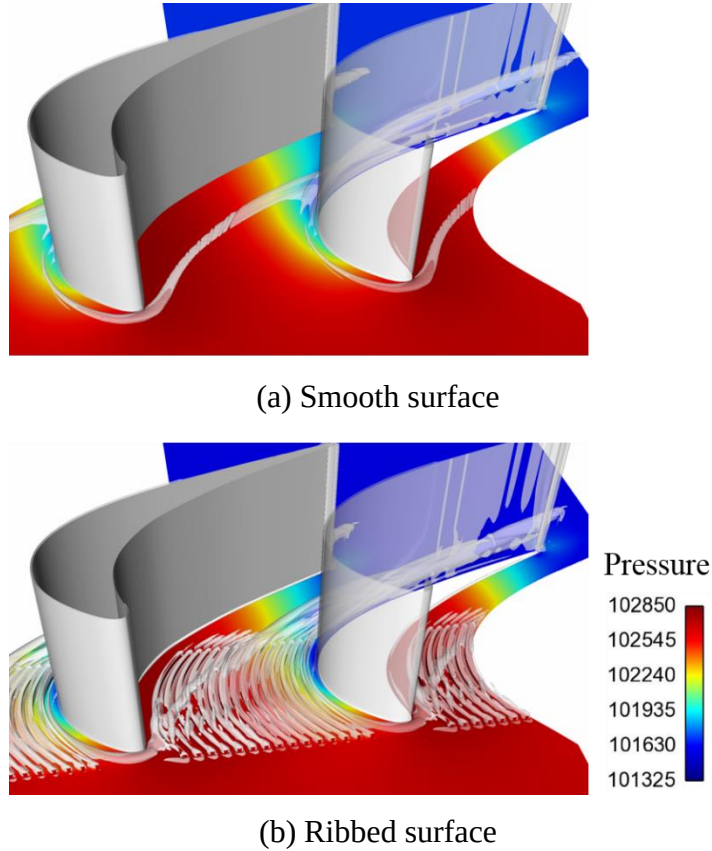
Figure 5.14: Iso-surfaces of \lambda_2 and pressure distribution for the smooth and ribbed surface.
