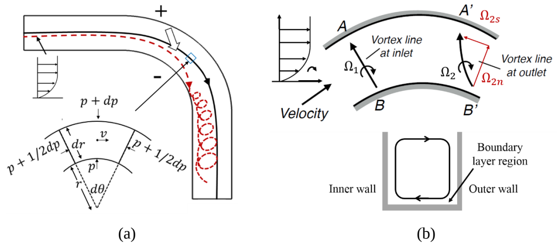
Figure 2.1: Generation of secondary flow in a curved duct (Modified by Greitzer et al. (2007)).
