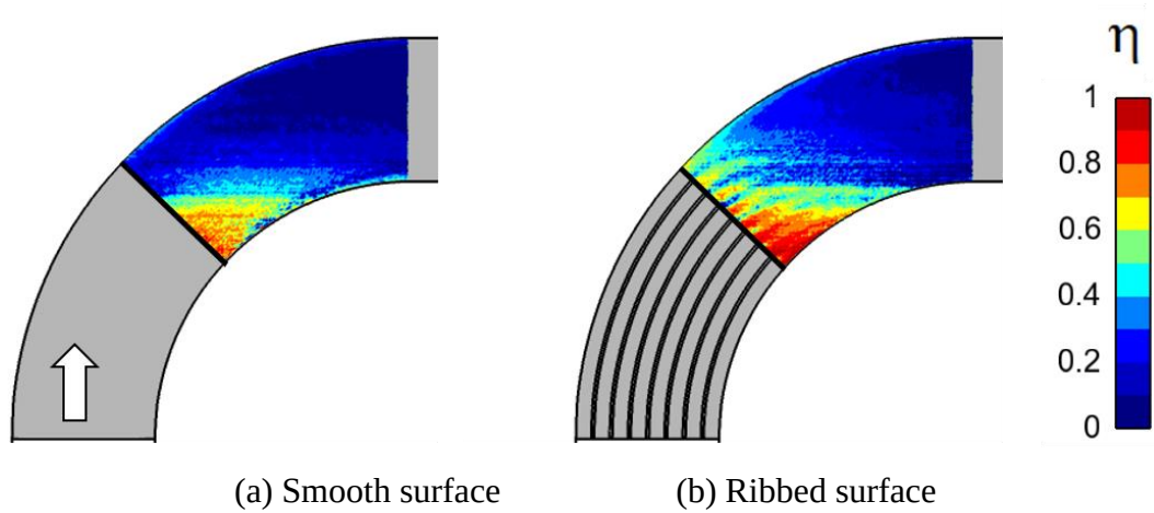
Figure 6.6: Film cooling effectiveness (experimental data).
