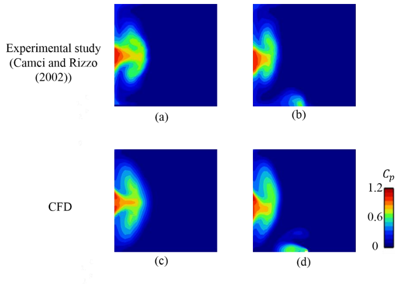
Figure 4.9: Total pressure loss coefficient C_p distributions for cases with and without single fence obtained at 90-degree plane of the duct.
