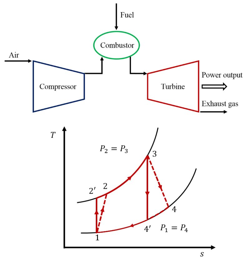
Figure 1.2: Simple gas turbine system and Brayton cycle.
