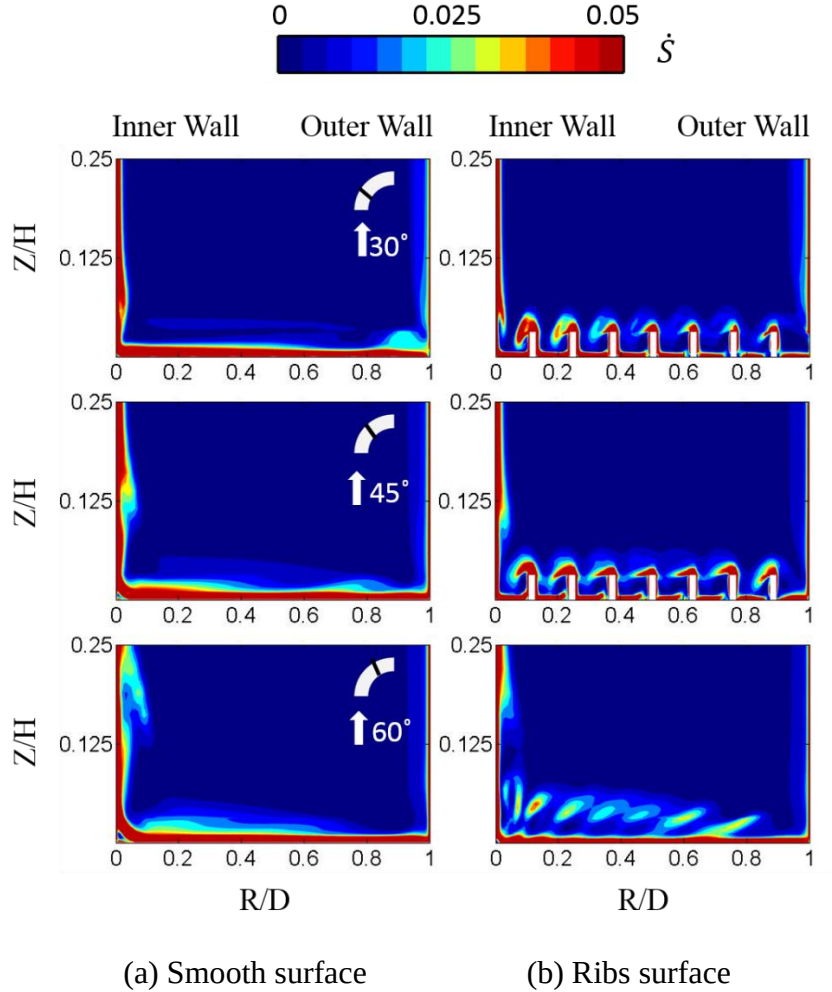
Figure 6.4: \dot{S} distributions at three angular cross sections.
