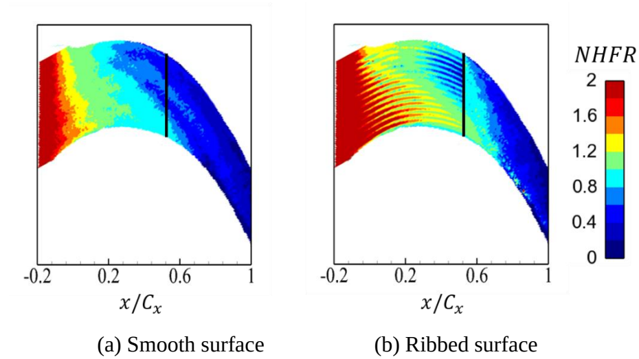
Figure 6.24: Distribution of NHFR. ( experimental data )
