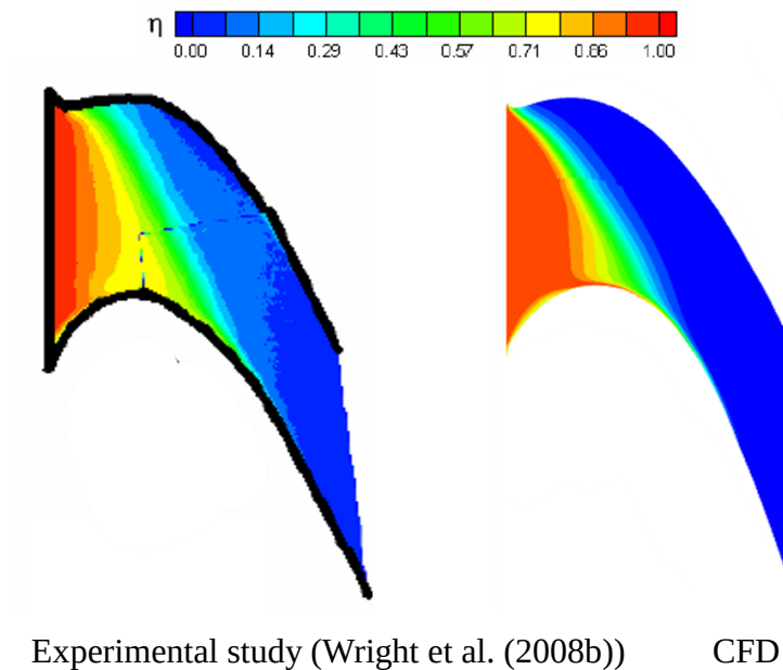
Figure 4.10: Film cooling effectiveness distributions on end-wall.
