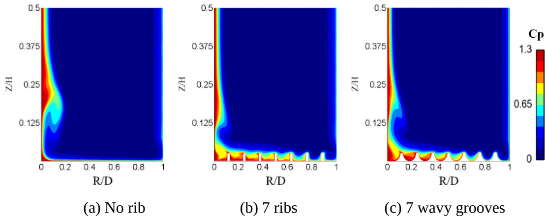
Figure 5.10: Aerodynamic loss coefficient C_p distribution at 90^\circ plane.
