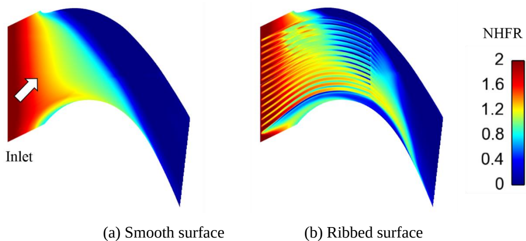
Figure 6.28: Distribution of NHFR in high-speed condition. (CFD results)
