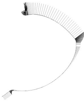
Fig 6. Clearance distribution between the rotors close to the rotor suction
