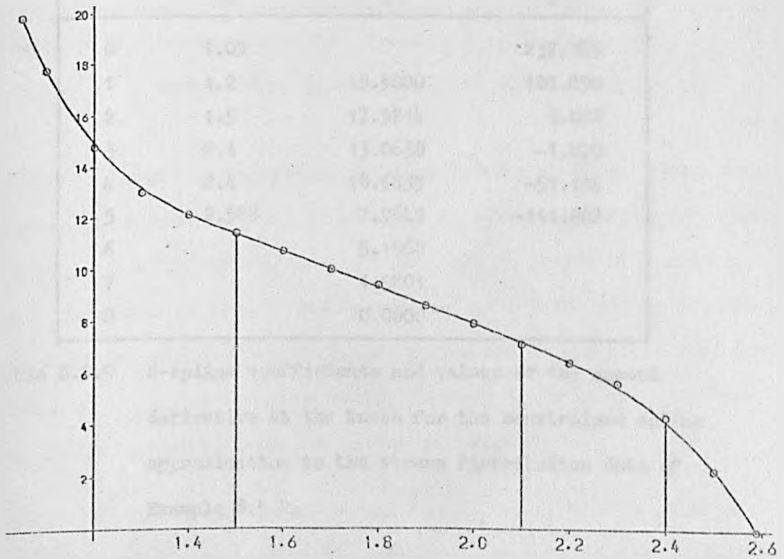
Fig 8.5.4 Stress distribution : S - shaped spline approximation
