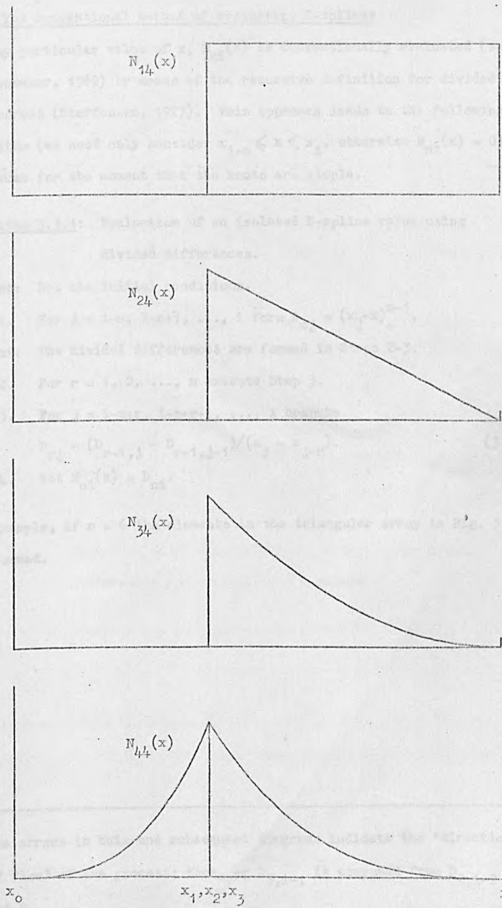
Fig. 3.2.2 The B-splines N_{14}(x) , N_{24}(x) , N_{34}(x) and N_{44}(x) with knots x_0 = 0 , x_1 = x_2 = x_3 = 0.4 and x_4 = 1 .
