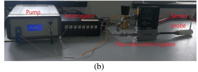
Fig. 2 Experimental set up: the sensor probe (left), the FBG wavelength change with heating (red) and cooling (blue) (top) and a photograph of the sensor probe showing its small size and compact packaging. (a) Schematic of the system and (b) Photograph of the actual device
