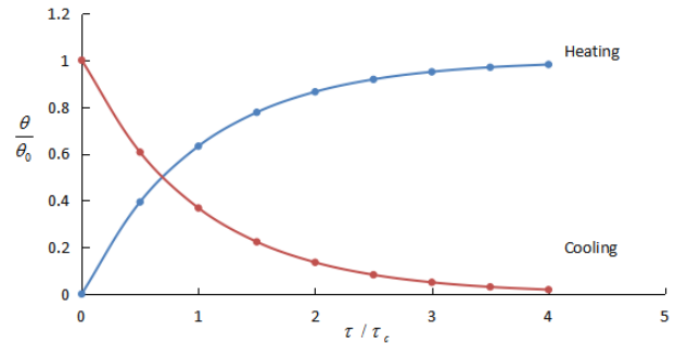
Fig. 1 The relationship between temperature and the normalized heating (blue) and the cooling (red) times
