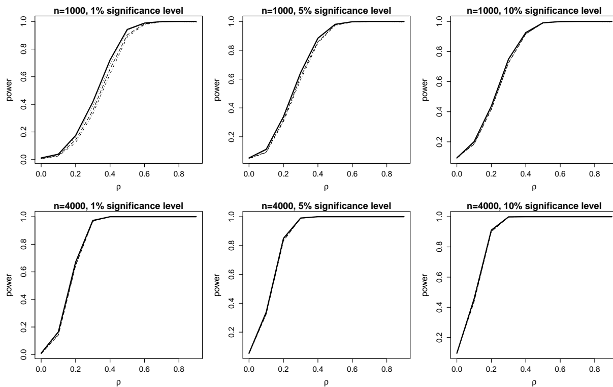
Figure 1: Rejection frequency curves for the LM (solid curve), W (dotted), G (dotdashed) and LR (long-dashed) tests. The results refer to the recursive model case when ER is present. Note that in almost all cases the curves differ only minimally, hence they can hardly be distinguished.
