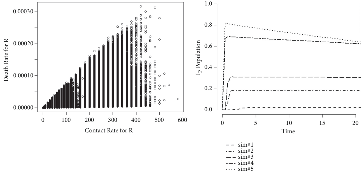
(a) Contact rate for R vs. death rate for R ( dh_R )
