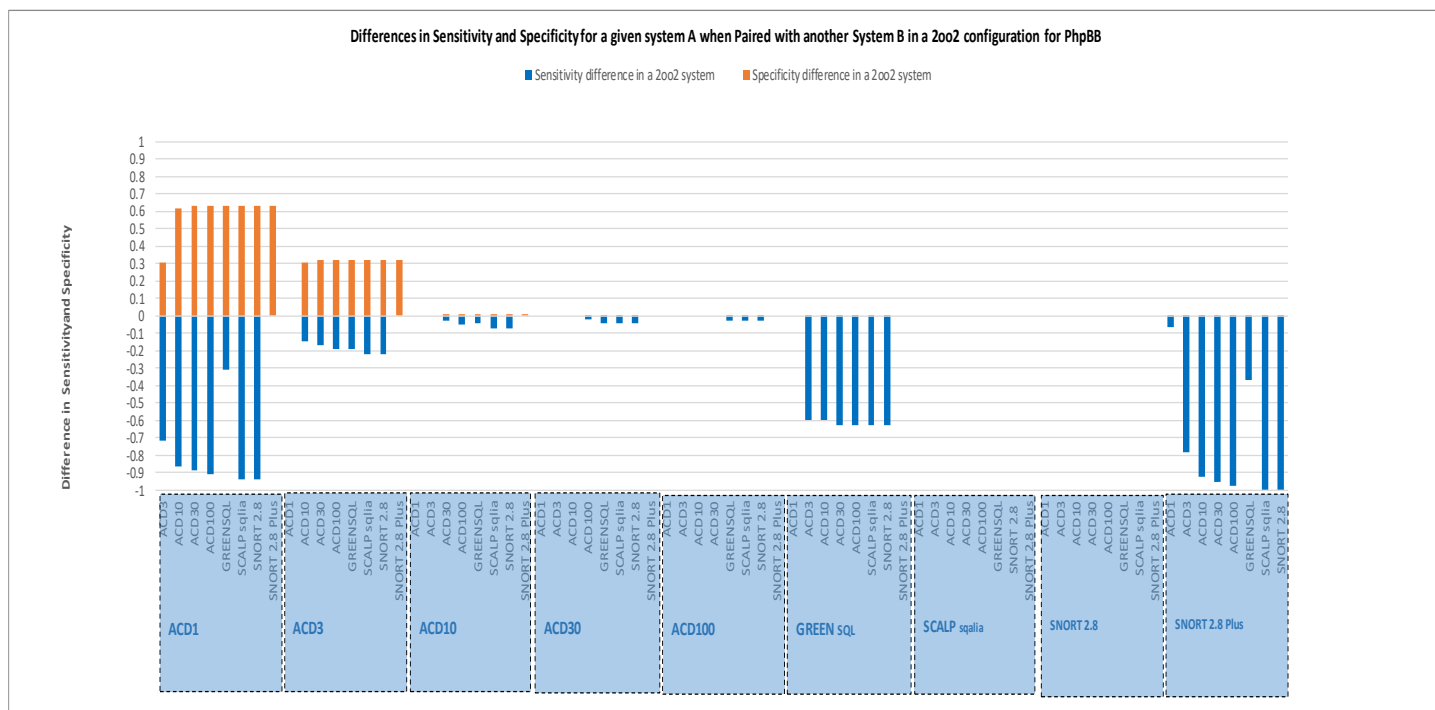
Figure 6-10 Differences in sensitivity and specificity for a given system A when paired with another System B for phpBB for a 2oo2 configuration
