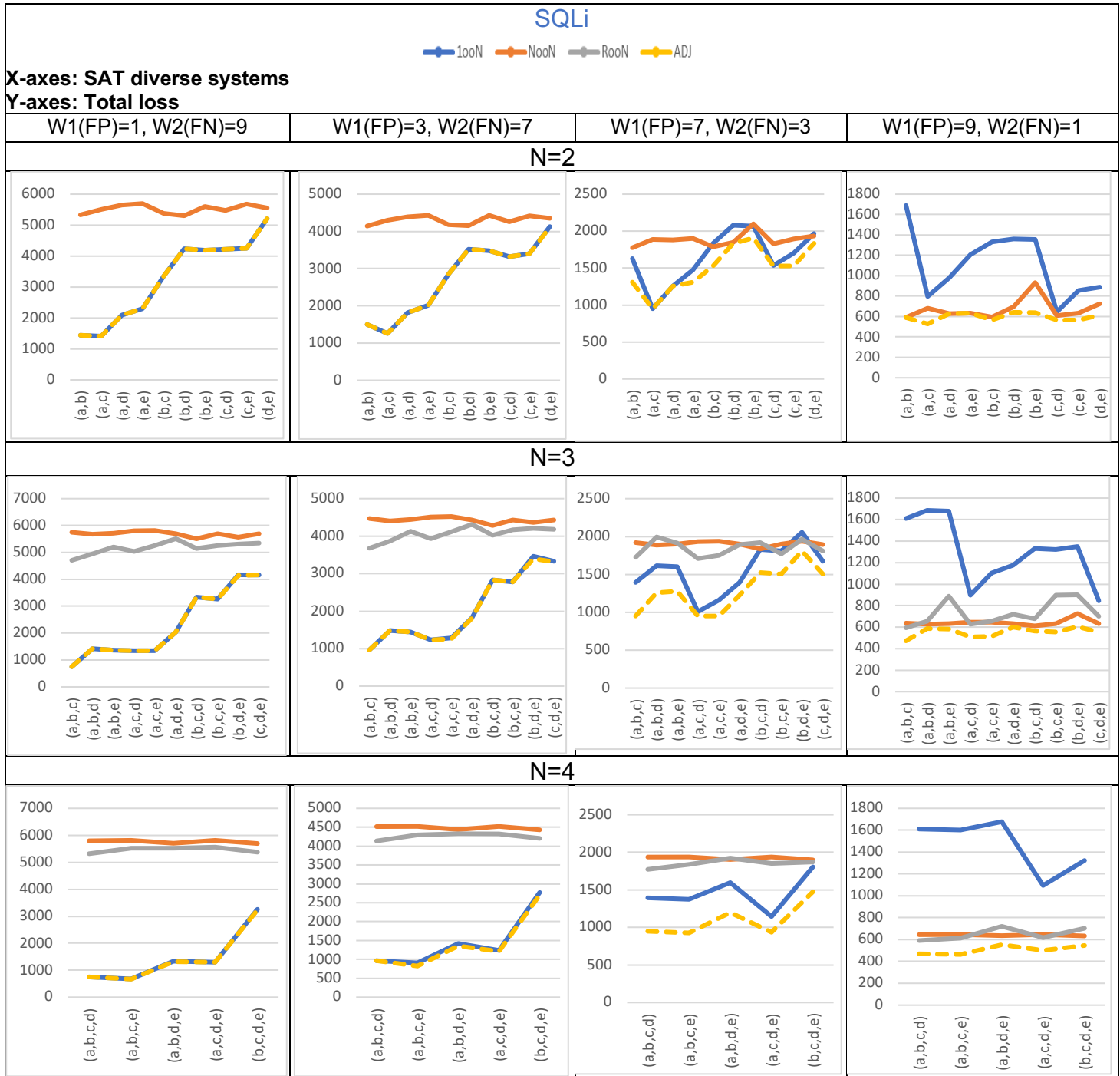
Appendix C-Figure 4 The weighted total loss (FP losses and FN losses) per diverse system configurations (10oN, majority vote, NooN and optimal adjudication) for (SQLi, N=2, 3 and 4)
