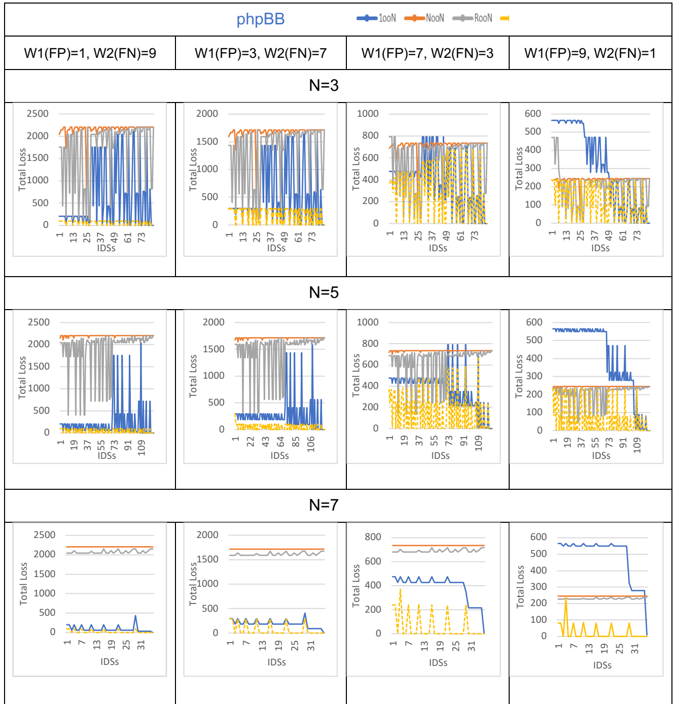
Appendix C-Figure 2 The weighted total loss (FP losses and FN losses) per diverse system configurations (100N, majority vote, NooN and optimal adjudication) for (phpBB, N=3, 5 and 7)
