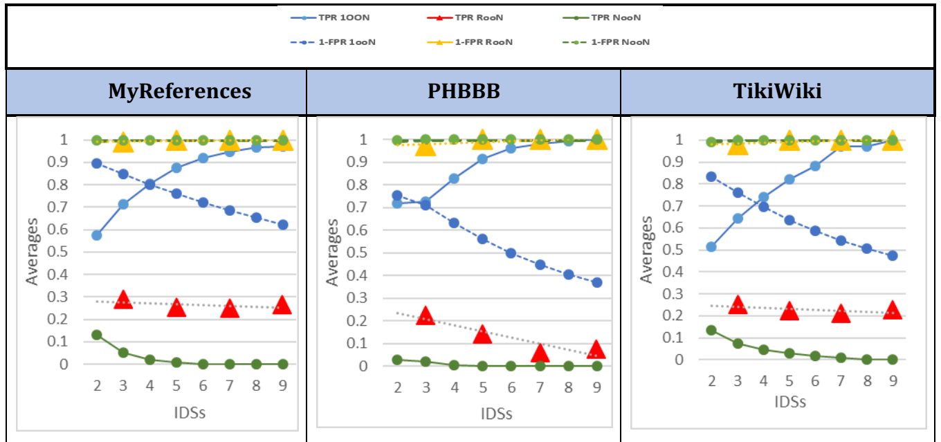
Figure 6-14 Plots show the averages of TPR and 1-FPR for the combined IDSs, in 100N, RooN and NooN configurations for all the web applications
