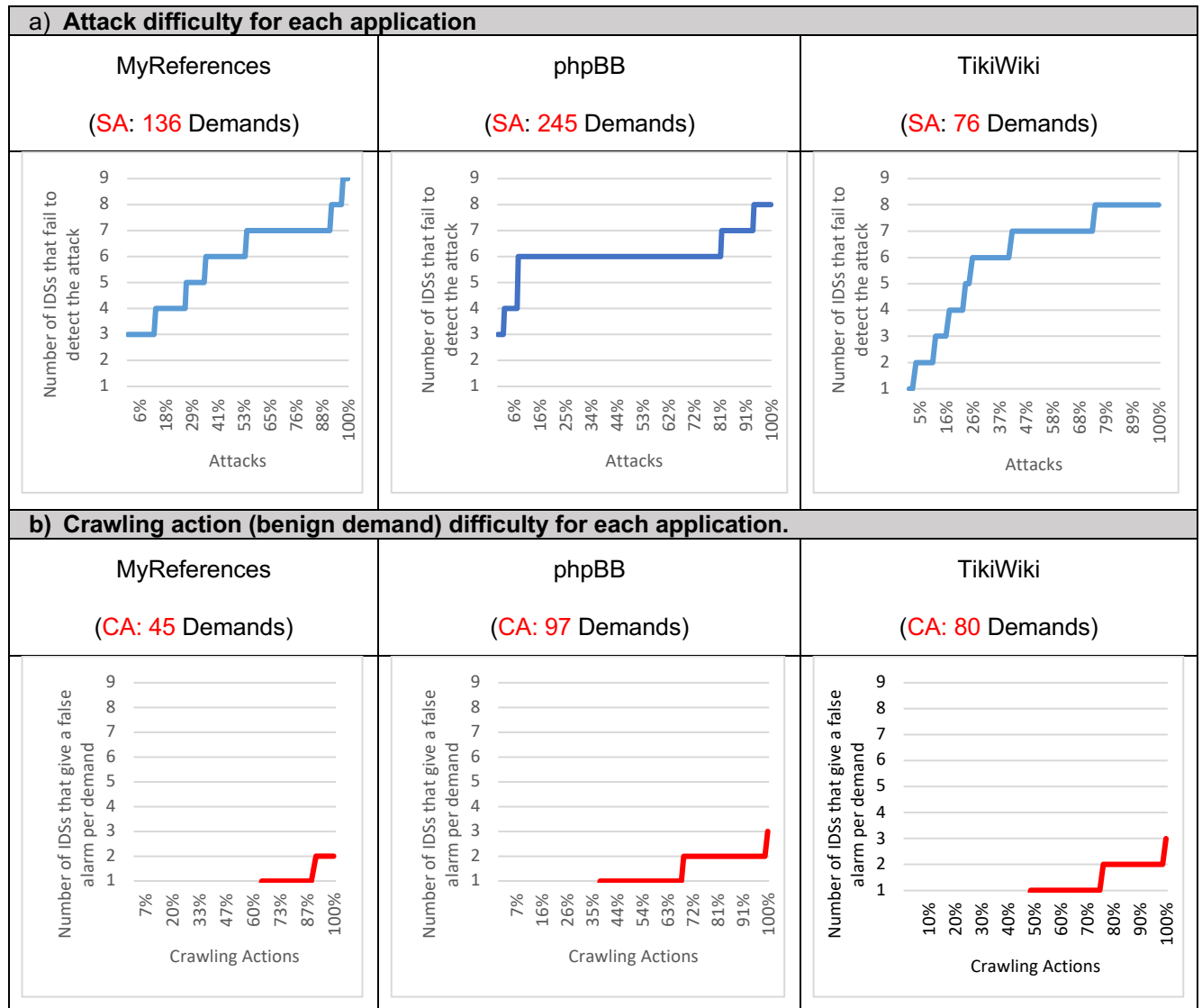
Appendix B. Figure 2 Demand difficulties of attack (a) and benign traffic (b) for each application.
