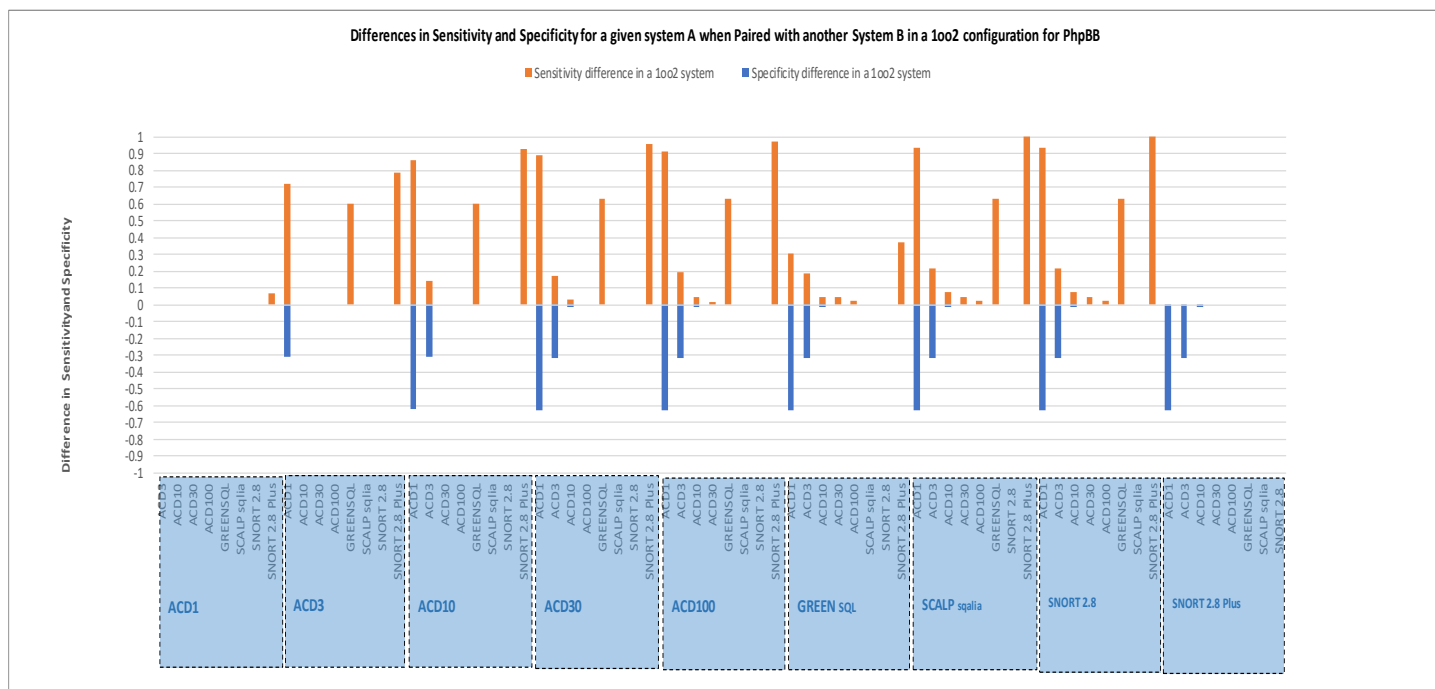
Figure 6-9 Differences in sensitivity and specificity for a given system A when paired with another System B for phpBB for a 1oo2 configuration
