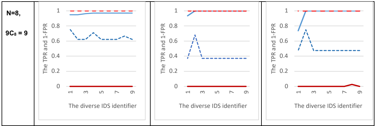
Appendix B. Figure 3 The TPR and 1-FPR Distribution Plots showing the combined IDSs, in 1ooN, RooN and NooN configurations. for each application ordered by TPR of 1ooN (so the x-value remains the same for each of the 6 lines on the plot). The x-axes represents the diverse IDSs for each configuration N.
