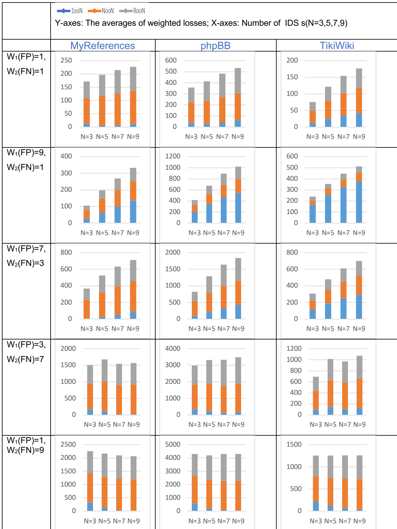
Figure 8-4 The average loss difference between the optimal adjudication function and the other diversity IDS setups ( 100N,majority vote and No0N) for each application. For N=3, 5, 7 and 9.
