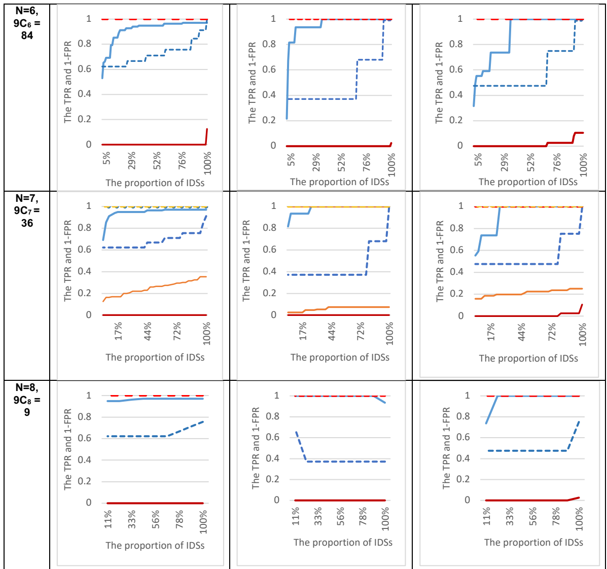
Appendix B .Figure 4 The TPR and 1-FPR Distribution Plots showing the combined IDSs, in 1ooN, RooN and NooN configurations. for each application ordered from low to high value. So each line is ordered from the best (left) to the worst (right), hence the actual value in the x-axis is not meaningful (though the proportion is).
