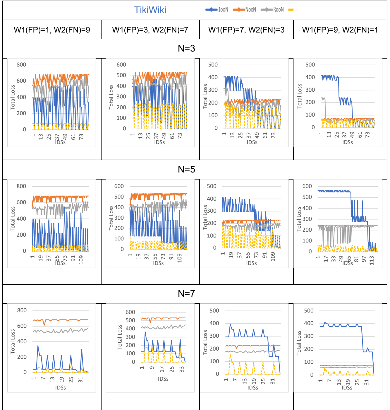
Appendix C-Figure 3 The weighted total loss (FP losses and FN losses) per diverse system configurations (100N, majority vote, No0N and optimal adjudication) for (TikiWiki, N=3, 5 and 7)
