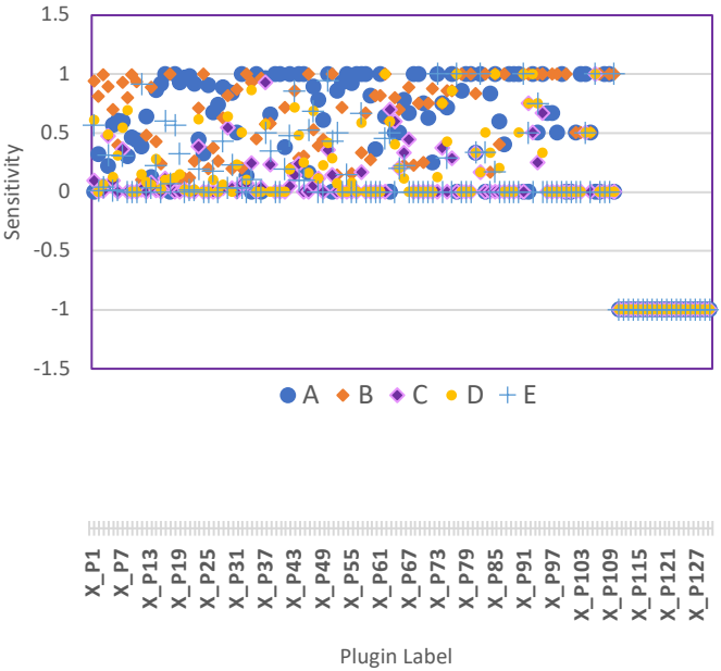
Figure 7-5 Vulnerable and non-vulnerable lines count per plugin and sensitivity measures, for SQLi and XSS.
