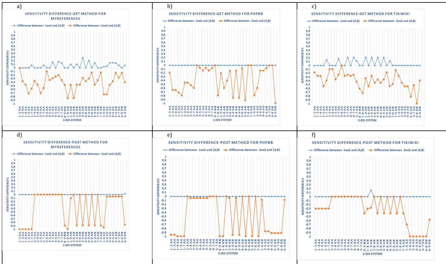
Figure 6-6 The sensitivity difference of 1002 and 2002 configurations compared with the best single system in the respective pair, charts a-c) show these differences for each application when attacks were Read (Get); whereas charts d-f), show them when they were Write (Post).
