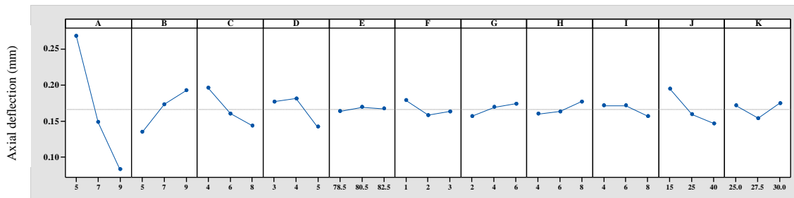
Figure 4. Effect diagram for sensitivity of axial deflection
