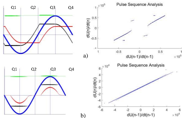
Figure 10. PD simulation over 50 cycles of the applied voltage, phase resolved data (left): PD pulses – green, applied voltage waveform – blue, voltage across the spark gap – black, voltage across the insulation – red; Pulse Sequence Analysis (PSA) plot (right); a) G_B = 5 \times 10^{-11} \text{S} ; b) G_B = 5 \times 10^{-6} \text{S}
