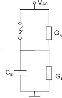
Figure 9. Equivalent circuit for PD simulation
