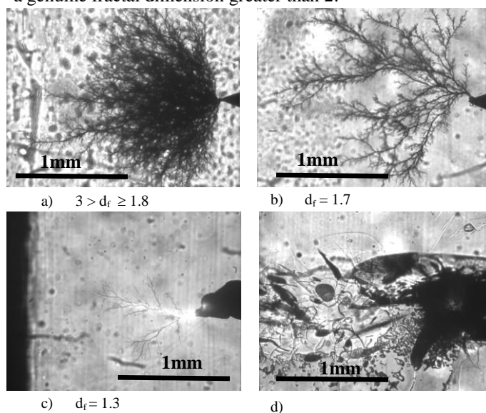
Figure 7. Electrical degradation and breakdown at different levels of absorbed moisture, temperature 20^\circ C , applied voltage 13.5kV rms, pin-plane distance 2mm: moisture level of: a) 0.1%, b) 1.0%, c) 2.4%, d) thermal breakdown at 6.9%. [18]
