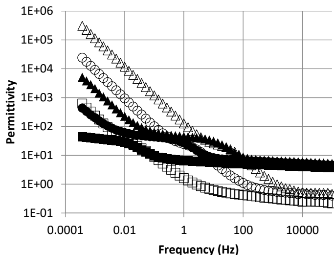
Figure 2. Real (filled) and imaginary (open markers) components of the relative permittivity of epoxy resin CY1311 at 20°C(■), 40°C(●), and 60°C(▲), absorbed moisture 0.1%, sample thickness 0.8 mm
