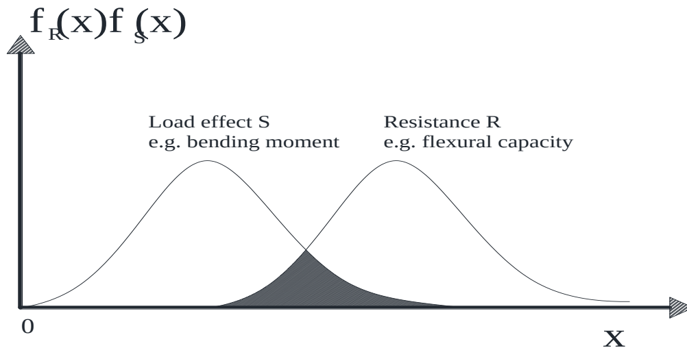
Figure C.2 Basic R-S problem: f_R() f_S() representation
