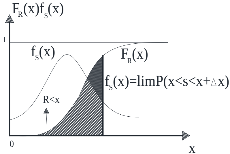
Figure C.1 Basic R-S problems: F_R() f_S() representation
