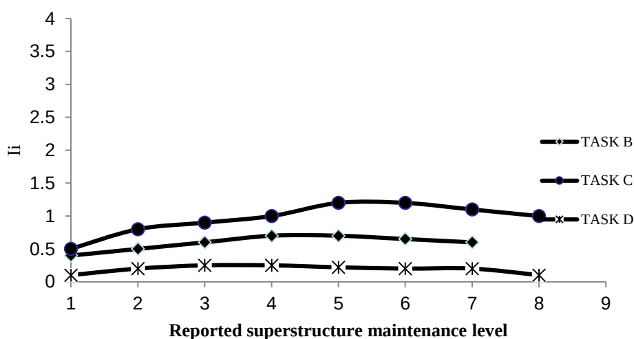
Figure 2.1b Inspection influence for condition rating on bridge superstructure with reported maintenance levels (Maintenance level: 1=very poorly, 9=very well) (AASHTO, 2001)
