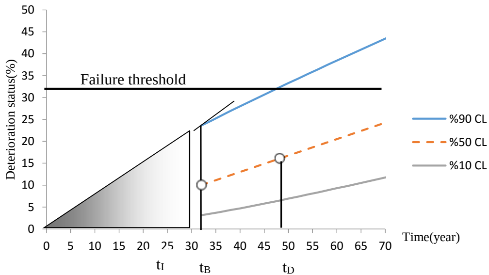
Figure 5.4 Deterioration status prediction graph based on prior inspection outcomes at age 18, 24 and 30
