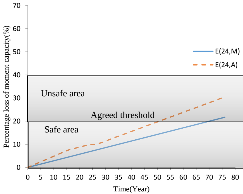
Figure 4.17 Comparison of predication of deterioration status based on the perfect and imperfect inspection type 2 at age 24(M=observed, A=actual)
