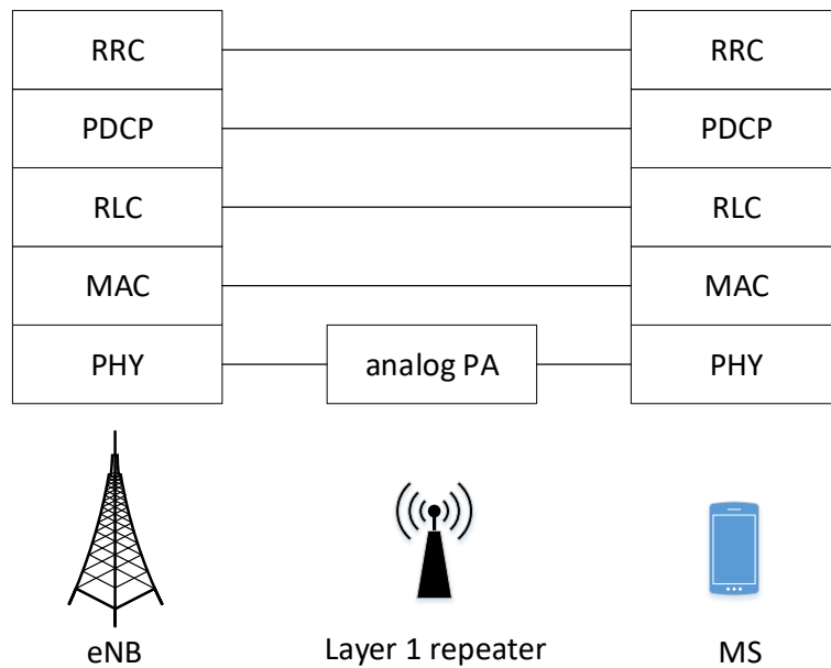
Figure 2.7: Layer 1 RN Protocol Stack
