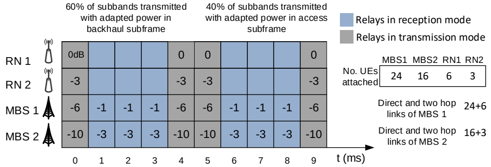
Figure 4.13: Numerical example of an optimized transmission power pattern
