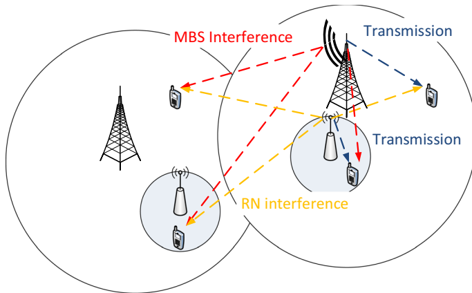
Fig. 2 Possible serving and interfering links during RN access transmission time
