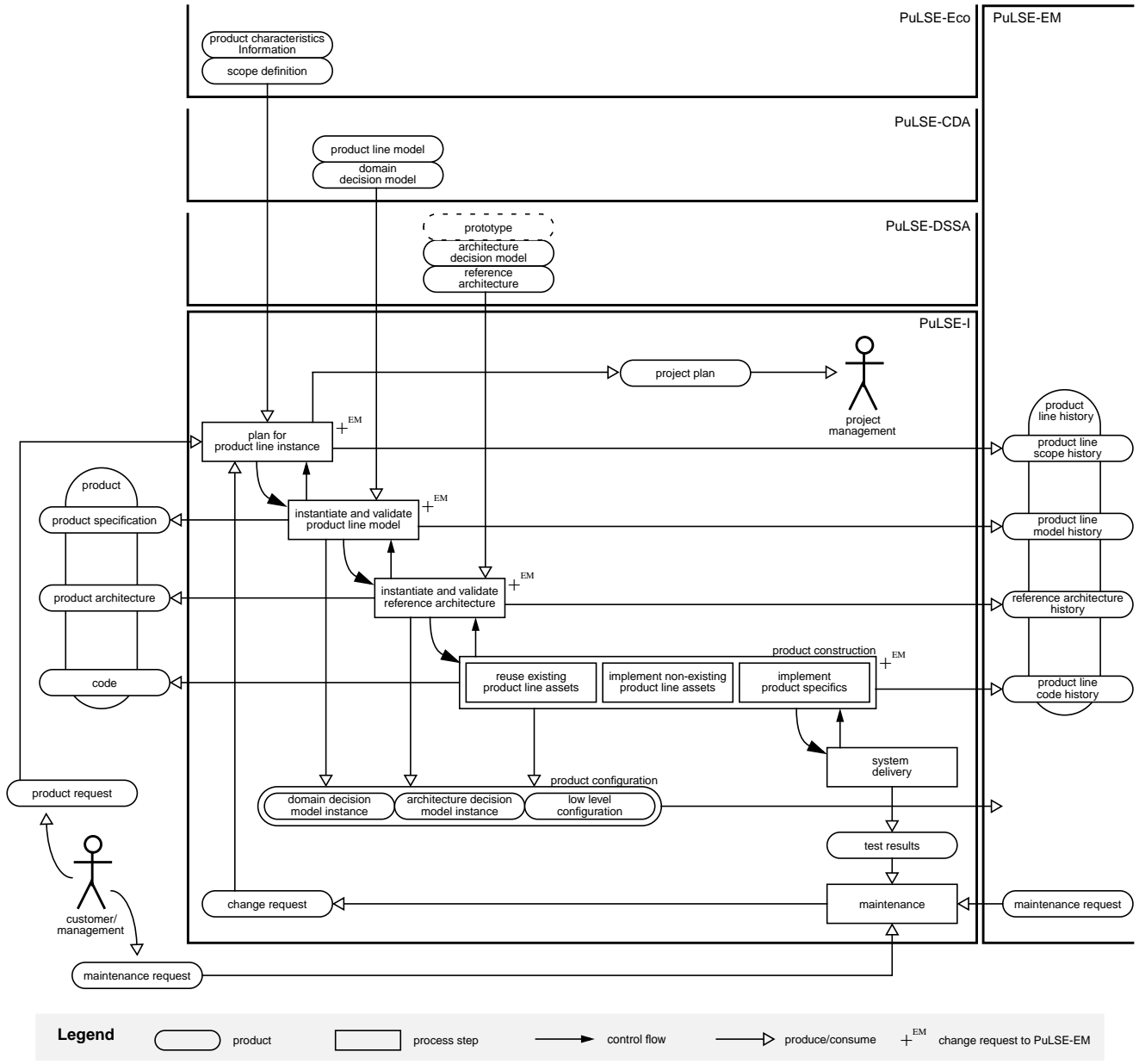
Figure 2. PuLSE-I Process
