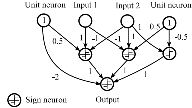
Fig. 3. Extended equality module
