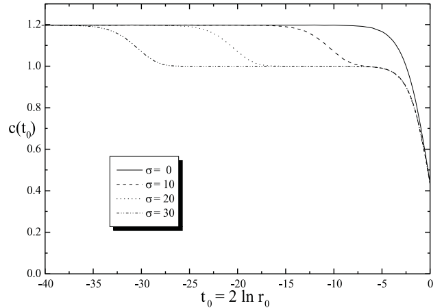
Figure 1: Renormalization group flow for the Virasoro central charge c(r_0) for various values of the resonance parameter \sigma .
