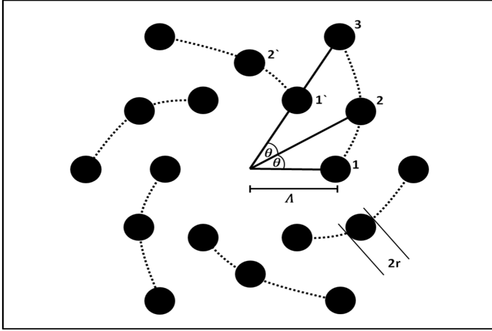
Fig. 1. Structure of the Equiangular Spiral-Photonic Crystal Fiber.
