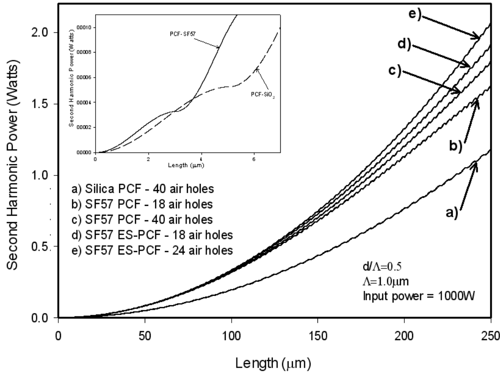
Fig. 9. Comparison of Quasi Phase Matched Second Harmonic output power with length, for different PCF structures and different materials. The inset graph shows an enlarged version of curves a) and c) for the propagation of a single coherence length.
