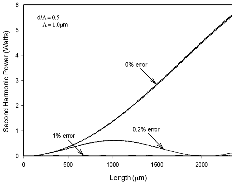
Fig. 8. Effect of fabrication tolerance on Second Harmonic output power with fifth order Quasi Phase Matching.
