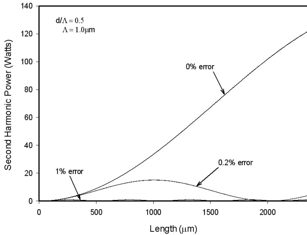
Fig. 7. Effect of fabrication tolerance on Second Harmonic output power with first order Quasi Phase Matching.
