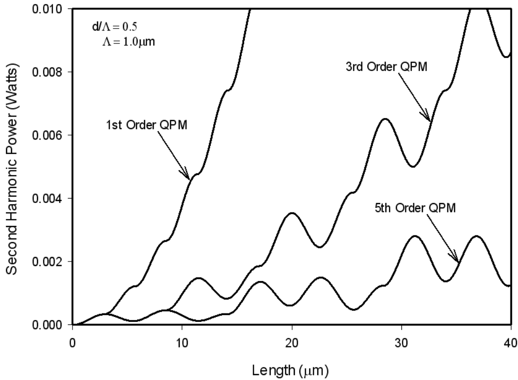
Fig. 6. Generated Second Harmonic power with first, third and fifth order Quasi Phase Matching.
