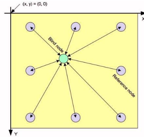
Fig. 5. Schematic diagram of the RSSI localization algorithm.
