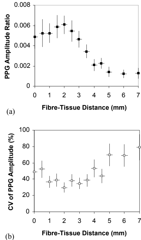
Figure 7: The effect of varying the distance d between the fibre ends and the tissue surface on (a) the PPG Amplitude Ratio and (b) the coefficient of variation of the PPG Amplitude Ratio. The fibre-fibre separation s was 2 mm.
