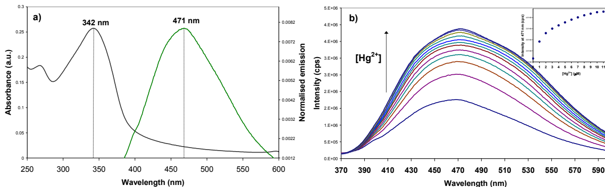
Figure 2. a) Absorption and emission spectra of CACE (10 \mu\text{M} ) in \text{H}_2\text{O}/\text{MeCN} (7:3, v/v). Emission spectrum recorded with \lambda_{\text{ex}} = 350 \text{ nm} . b) Emission spectra of CACE at [\text{Hg}^{2+}] ranging from 0 to 11 \mu\text{M} . The inset shows the titration plots at 471 nm ( \lambda_{\text{ex}} = 350 \text{ nm} ).
