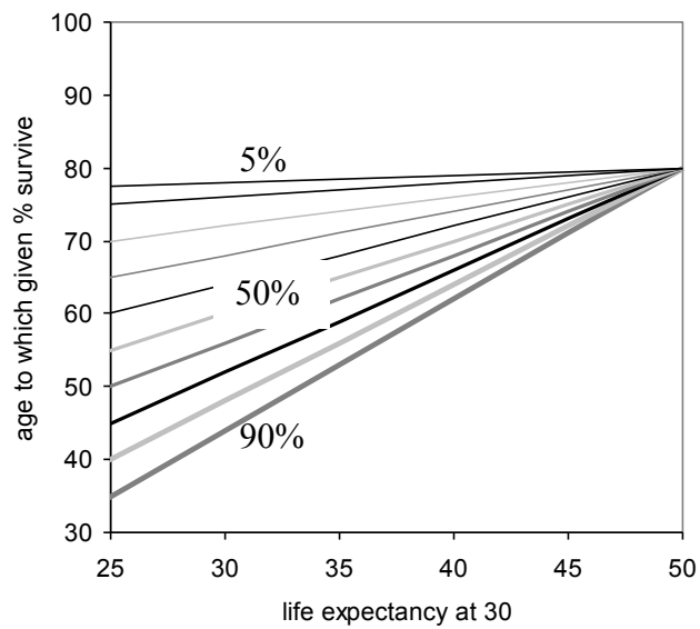
Figure B.2: Cumulative survival models: (a), (b) and (c)
