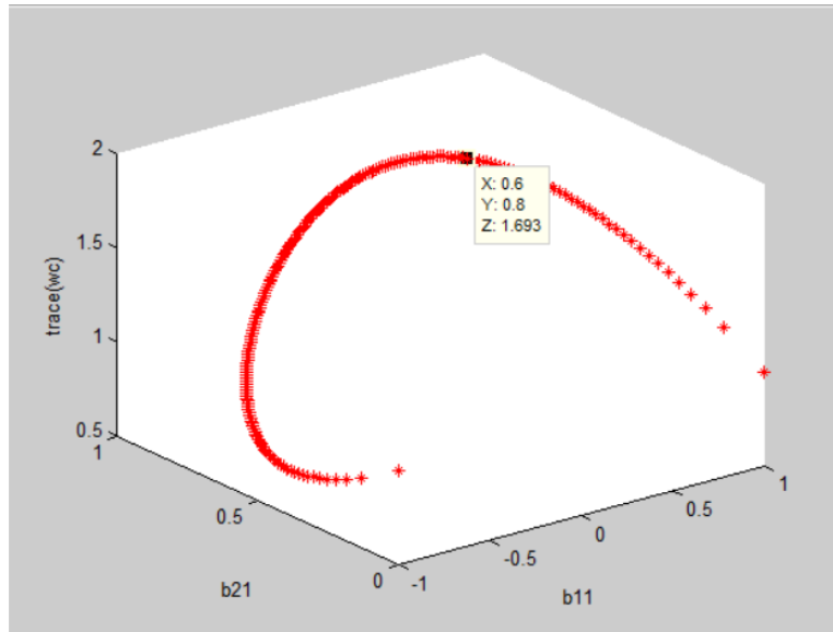
Figure (7.1): \text{trace}(W_c(0,1)) with respect to different values of b
