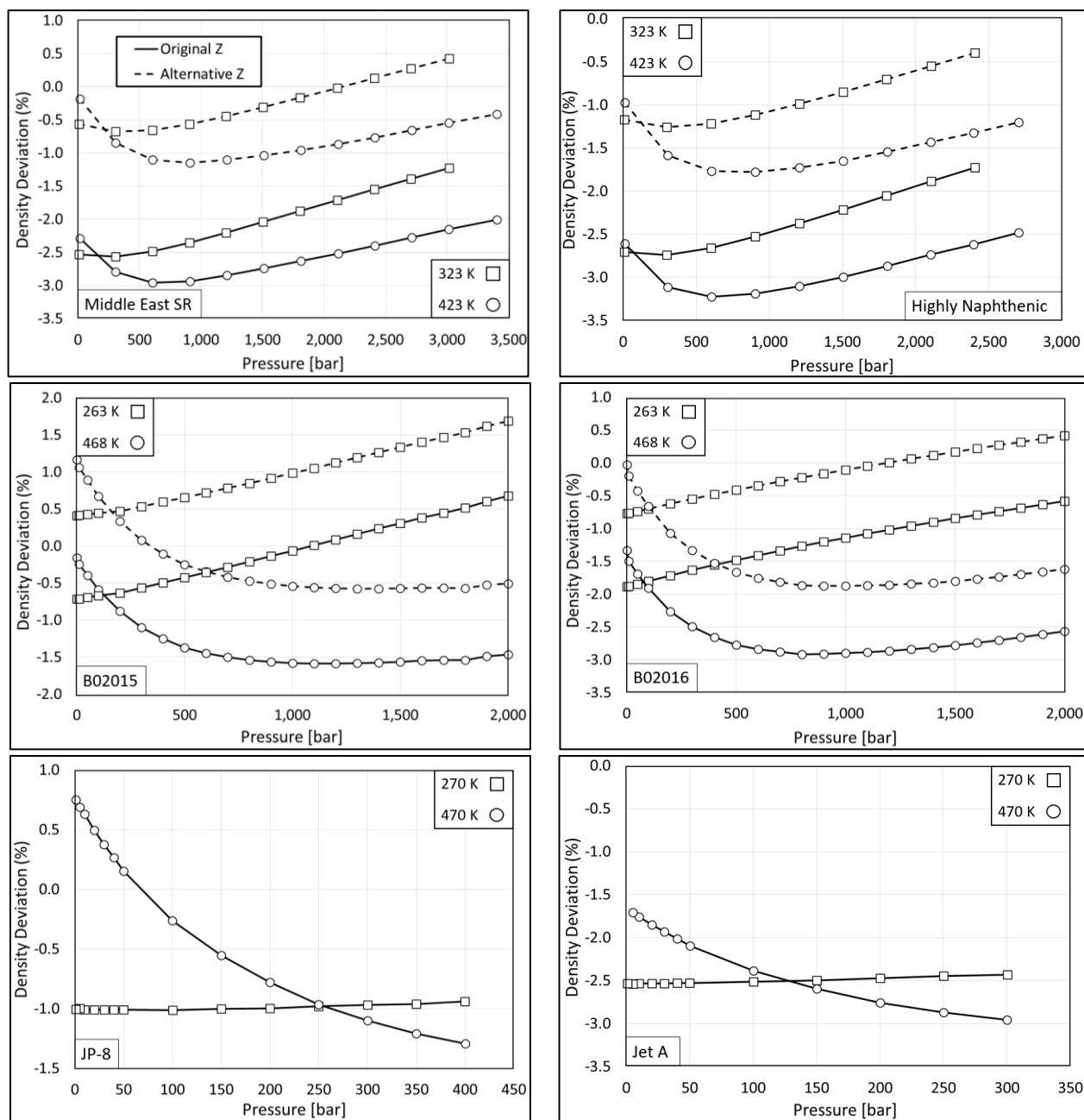
Figure 2.15. Predicted density deviations compared to experimental data [25, 140-142] for diesel and jet fuels. Lines are a guide for the eye.
