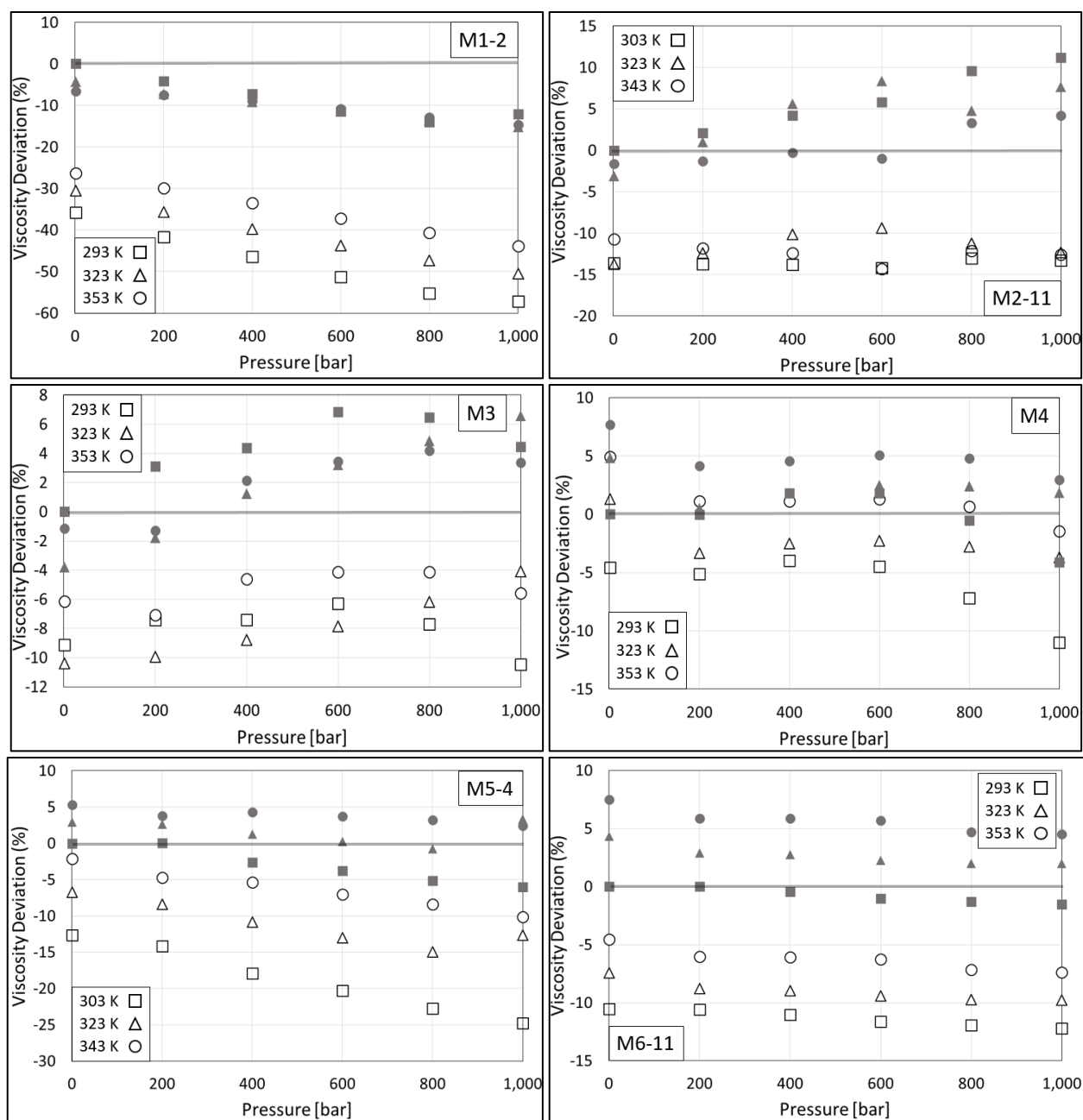
Figure 3.4. Pseudo-component viscosity deviations compared to experimental data [133, 185-188] for hydrocarbon mixtures listed in Table 3: two-parameter (open symbols) and three-parameter (filled symbols) models. Note that the y-axis scale is different in each figure.
