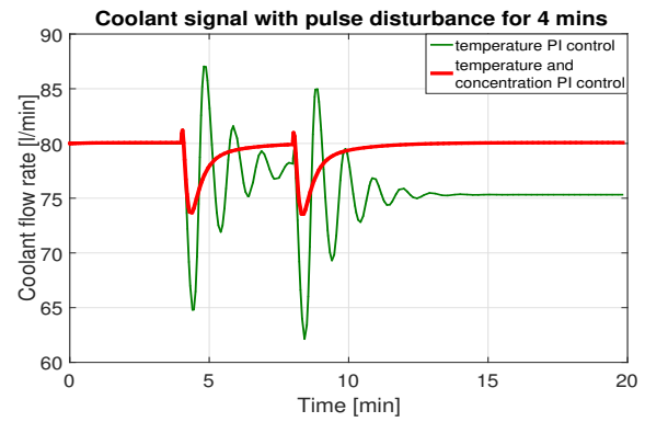
Figure 6. Coolant flow rate for temperature and both temperature and concentration PI control in the feeder.
