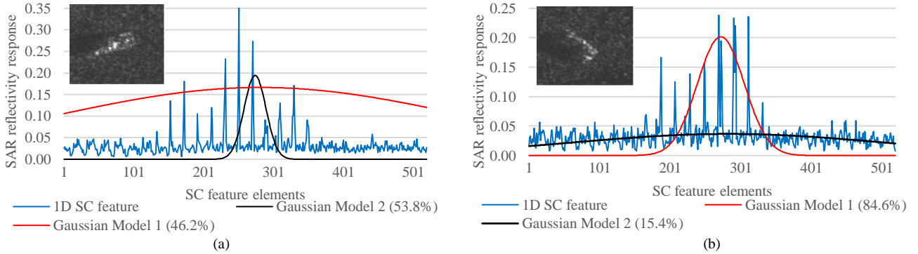
Fig. 1. GMM analysis of a SAR image (top left) in the 1D feature space showing (a) mutual GMM importance (b) dominant GMM importance (percentage highlights the influence per GMM distribution – GMMs scaled based on their % contribution)
