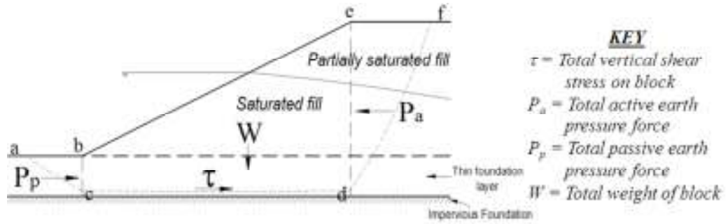
Figure 2.7 Application of Sliding Block Method for slope stability analysis
