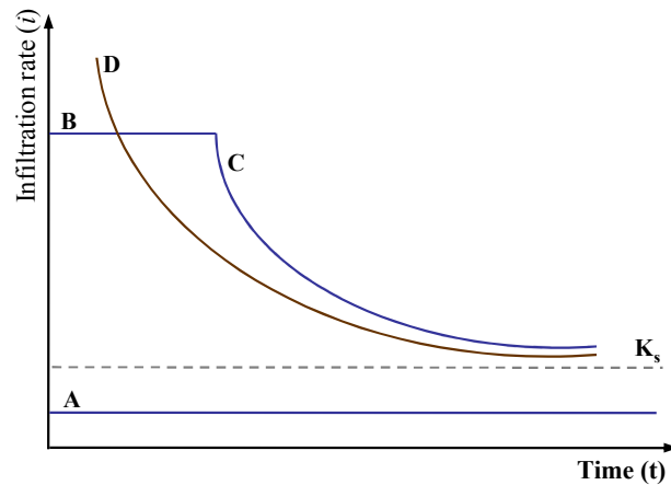
Figure 5.8 Sketch of infiltration rate as a function of time under different rainfall conditions
