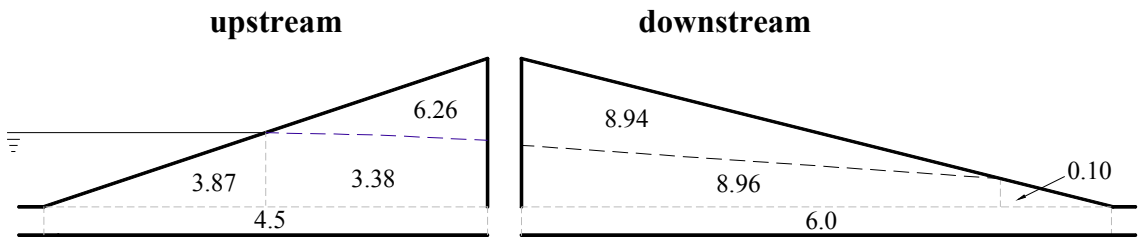
Figure 2.15 Areas (m 2 ) allocated within the upstream and downstream slopes and foundation
