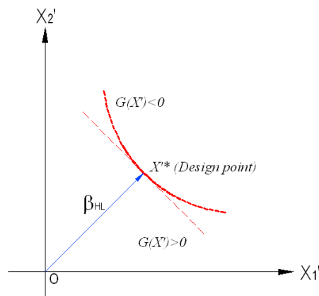
Figure 3.3. Hasofer-Lind reliability index for nonlinear limit state function in standard normal space
