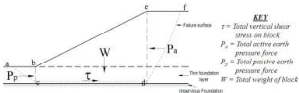
Figure 2.5 Sliding Block Method for analysis of slopes with a weak foundation layer
