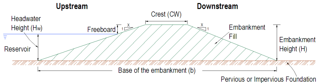
Figure 2.1 Cross sectional diagram of a homogeneous embankment
