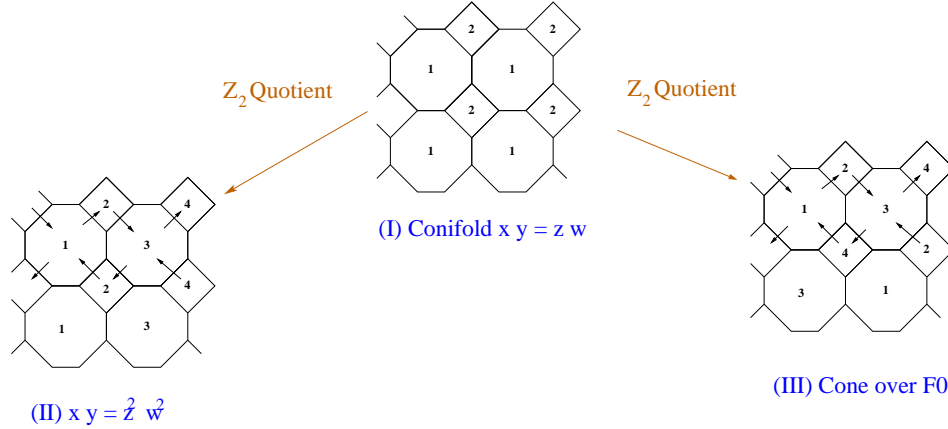
Figure 7: (I) Brane diamond for the conifold. Identifications in the infinite periodic array of boxes leads to a two-diamond unit cell, whose sides are identified in the obvious manner. From (I) we have 2 types of \mathbb{Z}_2 quotients: (II) Brane diamond for the \mathbb{Z}_2 quotient of the conifold xy = z^2 w^2 , which is a case of the so-called generalised conifold. The identifications of sides are trivial, not tilting. The final spectrum is the familiar non-chiral spectrum for a brane interval with two NS and two NS' branes (in the alternate configuration); (III) Brane diamond for the \mathbb{Z}_2 quotient of the conifold yielding the complex cone over F_0 . The identifications of sides are shifted, a fact related to the specific 'tilted' refinement of the toric lattice.
