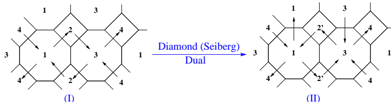
Figure 6: Seiberg duality from the brane diamond construction for the generalized conifold xy = z^2w^2 . Part (I) corresponds to the brane interval picture with alternating ordering of NS- and NS'-branes, whereas part (II) matches the other ordering.
