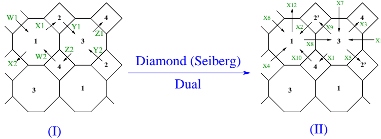
Figure 8: Brane diamond for the two cases of the cone over F_0 . (I) is as in Figure 7 and (II) is the result after the diamond duality. The resulting spectrum and interactions are those of the toric dual (and also Seiberg dual) of the initial theory (I).
