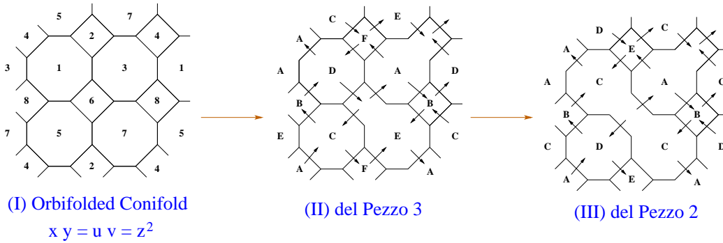
Figure 10: (I) Brane diamond for a \mathbb{Z}_2 \times \mathbb{Z}_2 orbifold of the conifold, namely xy = z^2 ; uv = z^2 . From this we can partial resolve to (II) the cone over dP_3 and thenceforth again to (III) the cone over dP_2 , which we shall discuss in the context of Seiberg duality.
