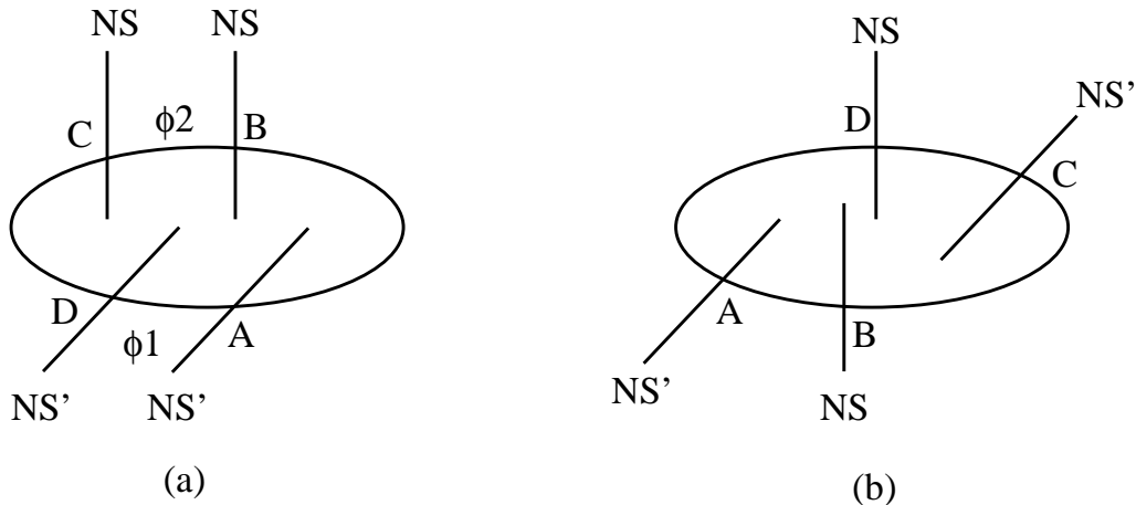
Figure 1: The two possible brane setups for the generalized conifold xy = z^2w^2 . They are related to each other passing one NS-brane through an NS'-brane. A_i, B_i, C_i, D_i i = 1, 2 are bifundamentals while \phi_1, \phi_2 are two adjoint fields.
