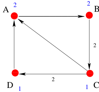
Figure 14: A non-Abelian phase of the complex cone over dP_3 . This example is Picard-Lefschetz dual to the other 4 examples in Figure 12 but not Seiberg dual thereto.
