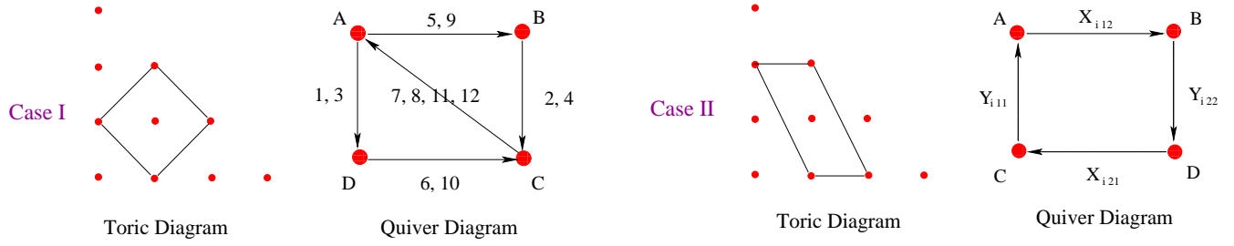
Figure 4: The quiver and toric diagrams of the 2 torically dual theories corresponding to the cone over the zeroth Hirzebruch surface F_0 .
