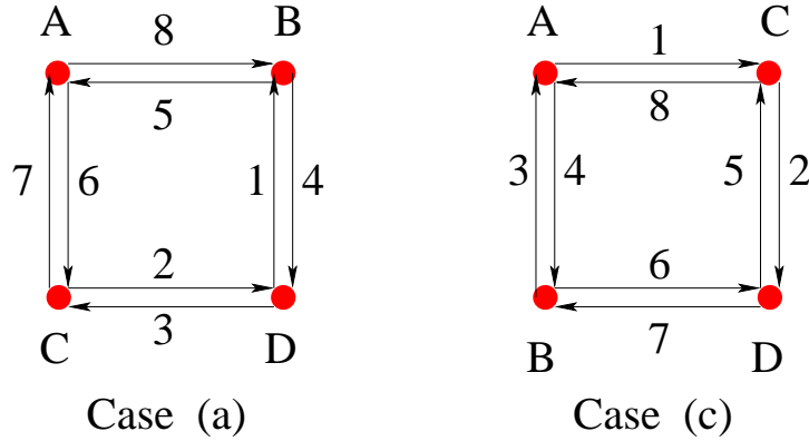
Figure 3: The quiver diagram encoding the matter content of Cases (a) and (c) of Figure 2.
