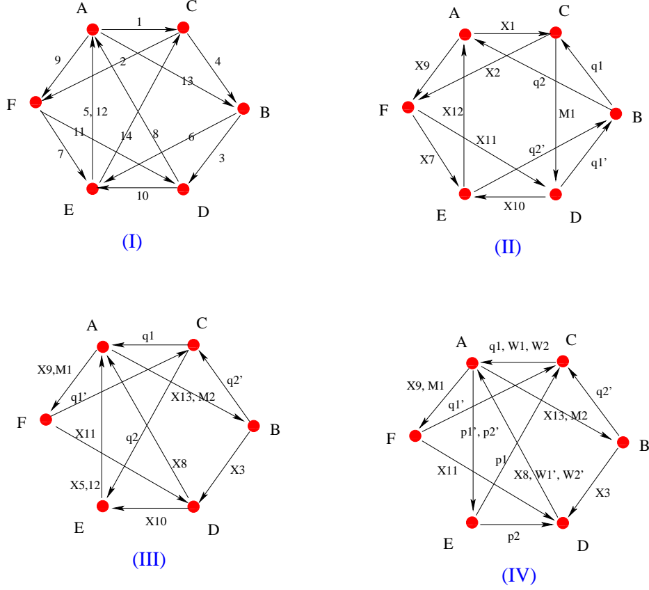
Figure 12: The four Seiberg dual phases of the cone over dP_3 .
