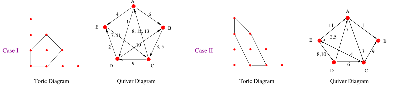
Figure 5: The quiver and toric diagrams of the 2 torically dual theories corresponding to the cone over the second del Pezzo surface.
