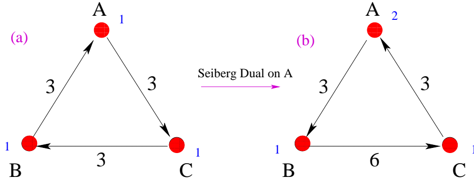
Figure 13: Seiberg Dualisation on node A of the \mathbb{C}^3/\mathbb{Z}_3 orbifold theory. The subsequent theory cannot be obtained by a Picard-Lefschetz monodromy transformation.
