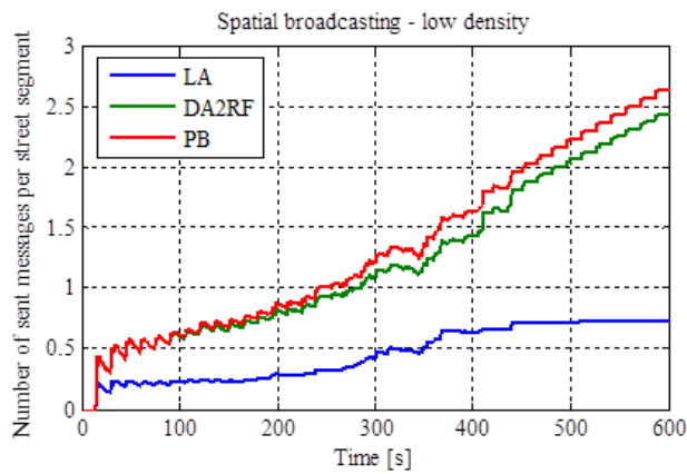
Figure 5.12: Spatial Communication in low density scenario for the LA , DA2RF and PB mechanisms.
