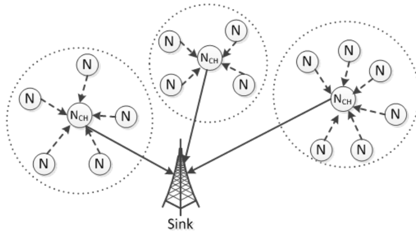
Figure 3.1: Cluster-based aggregation.
