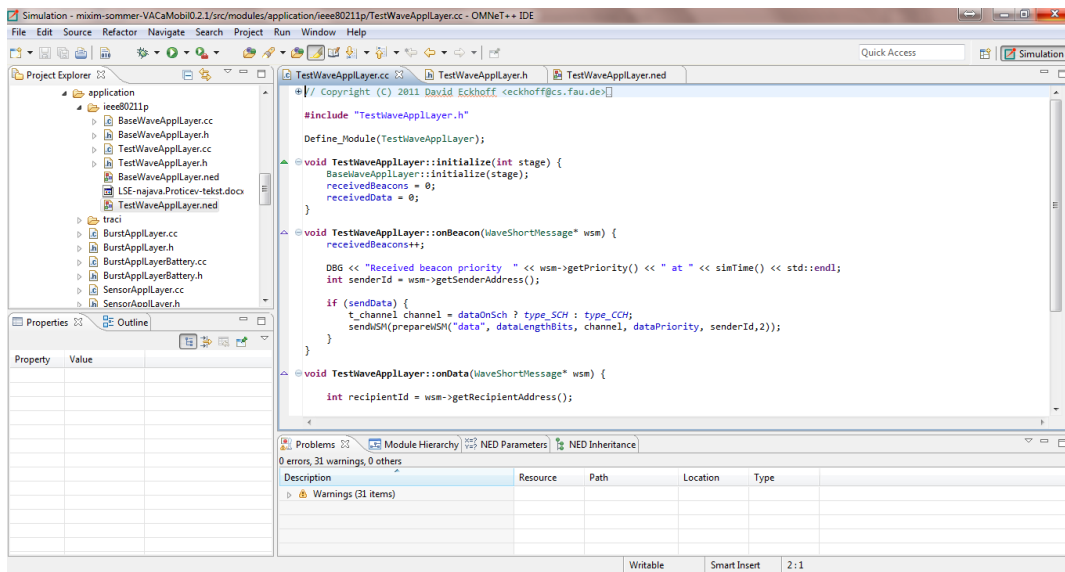
Figure 5.3: OMNeT++ screenshot.
