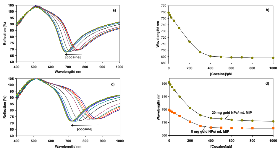
Figure 3. Response of the sensors to cocaine in the concentration range from 0 to 1000 \mu\text{M} . a) SPR spectra of sensor 1 - MIP with embedded gold NPs (8 mg/ mL MIP). b) Plot showing the dependence of SPR wavelength on cocaine concentration for sensor 1. c) SPR spectra of sensor 2 - MIP with embedded gold NPs (20 mg/ mL MIP) d) Plots showing the dependence of SPR wavelength on cocaine concentration for sensors 1 and 2.
