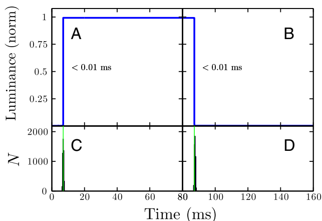
Fig. 10 a, b Response time curves, averaged over 10,000 off-on ( a ) or on-off ( b ) transition. Individual measurements were aligned temporally via crosscorrelation prior to averaging. Panels c and d show the distribution of cross-correlation lag times (i.e., amount of trial-by-trial lateral variability in the response curve shown above). The shape of the curves in the upper panels indicates the response time. The distributions in the lower panels indicate mean onset lag (green vertical line), and variability in onset lag (histograms)
